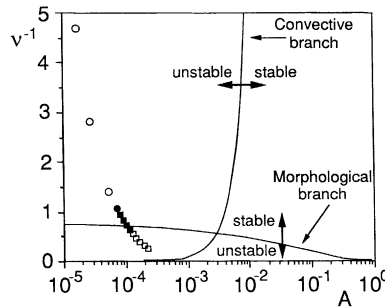
Fig. 2. — Diagram of solutal convection in the liquid phase superimposed on the basic diagram v^{-1} versus A for morphological instability of a planar solidification front. Experimental points : (○) no microstructure ; (●) elongated cells ; (■) cells ; (□) dendrites.
