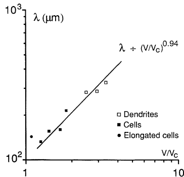
Fig. 7. — Variation of the primary spacing \lambda with V/V_C .
