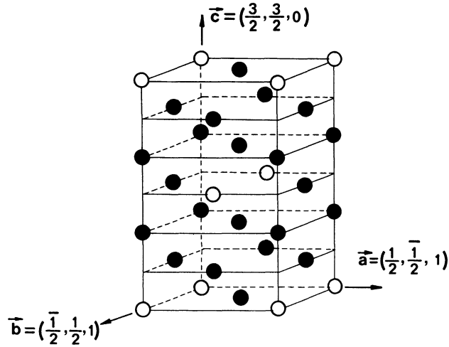
Fig. 11. — A_5B structure (orthorhombic unit cell). (O) : B atoms (vacancy) ; (●) A atoms (nitrogen). \mathbf{a} // \langle 1\bar{1}2 \rangle_{\text{fcc}} , \mathbf{b} // \langle \bar{1}12 \rangle_{\text{fcc}} , \mathbf{c} // \langle 110 \rangle_{\text{fcc}} . For each orthorhombic unit cell vector \mathbf{a} , \mathbf{b} , \mathbf{c} , are indicated its components in the disordered f.c.c. cell.
