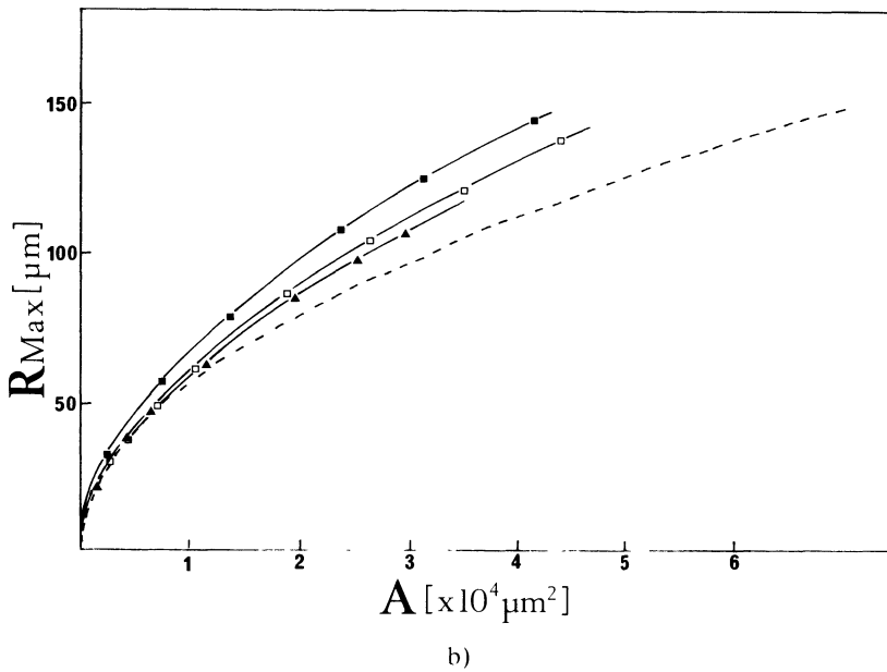
Fig. 6. — Global properties of a germ in the petal shape regime ; a) total area versus time ; b) maximum radius of the germ versus its area (the dotted line corresponds to a circular germ).
