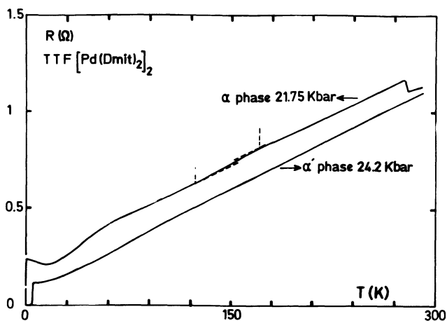
Fig. 3. — Compared temperature dependence of the resistances of \alpha and \alpha' -TTF [\text{Pd}(\text{dmit})_2]_2 phases at high pressures (measured at low temperatures).
