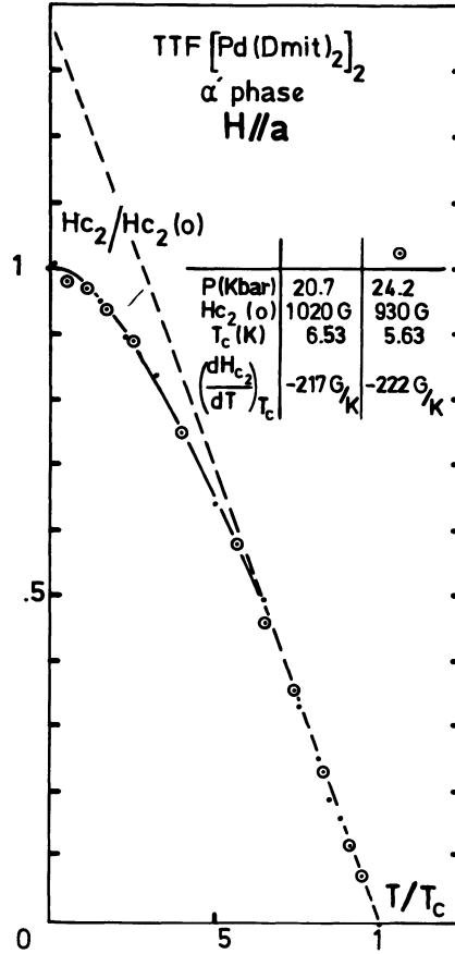
Fig. 6. — Temperature dependence of the reduced critical field h_{c_2} = H_{c_2}(T)/H_{c_2}(0) at two pressures. The magnetic field H is directed along the a axis of the unit cell of \alpha' -TTF [Pd(dmit) _2 ] _2 . The H_{c_2}(0) values are experimental. The values of T_c and of (dH_{c_2}/dT)_{T_c} were obtained by high temperature linear regression.
