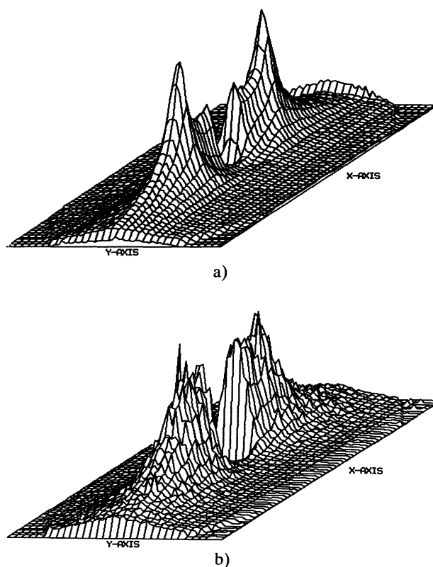
Fig. 7. — a) 2D scattering pattern of a CPCI L_\alpha mixture with d : 200 \text{ \AA} (neutrons) sample to detector distance : 2.5 m. b) 2D scattering pattern of a CPCI L_\alpha mixture with d : 970 \text{ \AA} (neutrons); sample to detector distance : 10.5 m.
