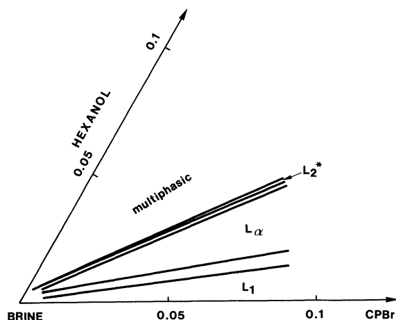
Fig. 2. — Brine rich corner of the phase diagram of the system CPBr/hexanol/brine.
