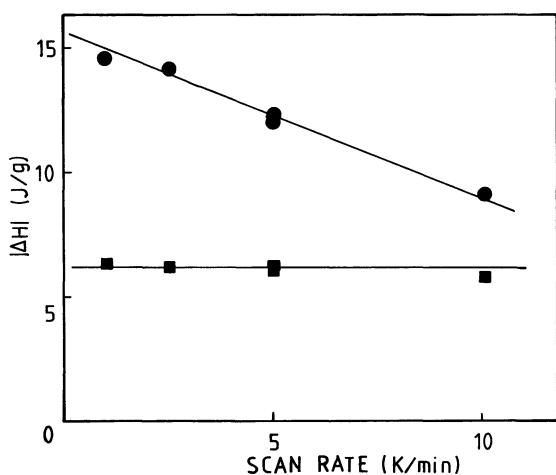
Fig. 4. — Transition enthalpies for PM-1 (RP23) as a function of the cooling rate ; filled squares correspond to the 120 \text{ °C} peak, for the « glass transition » ; filled circles correspond to the 137 \text{ °C} peak, for the liquid crystal-isotropic melt transition.
