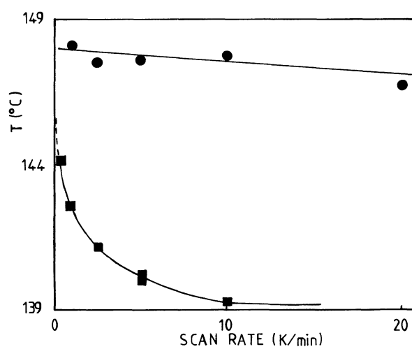
Fig. 2. — DSC peak onsets as a function of scan rate for the PM-2 polymer; filled circles and squares indicate heating and cooling scans respectively.
