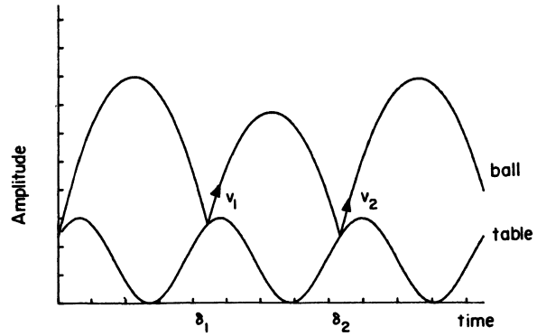
Fig. 5. — Ball and table position from numerical simulation. The phase and velocity variables are related by elementary considerations of projectile motion. The numerical simulation shows that the phase of impact can not be neglected when computing the time of flight between impacts.
