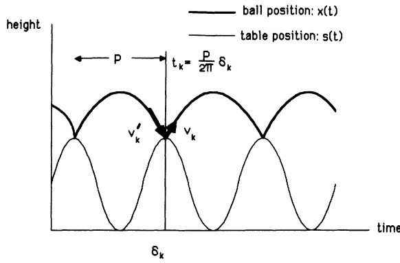
Fig. 2. — Ball and table position. Period motion of period P is depicted. Prime denotes ingoing velocity.
