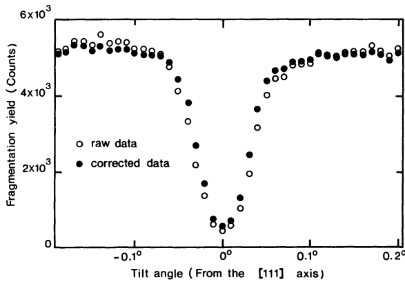
Fig. 3. — Angular scan of the fragmentation product yield across the [111] axis : (O) raw data, (●) corrected data (see text). Angular step : 0.01^\circ per channel.
