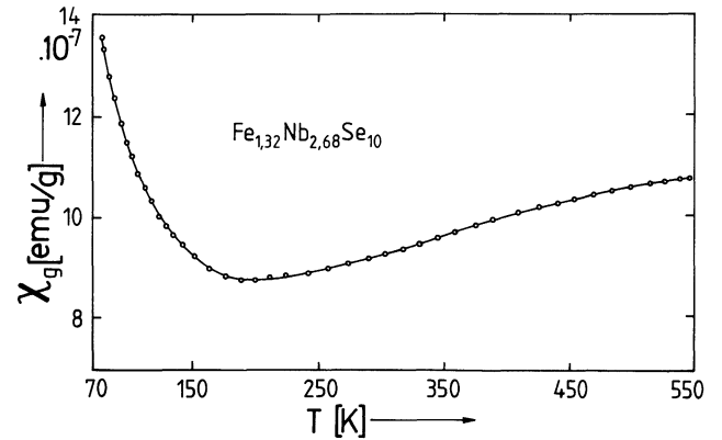
Fig. 5. — Temperature dependence of the magnetic susceptibility for \text{Fe}_{1,32}\text{Nb}_{2,68}\text{Se}_{10} powder.
