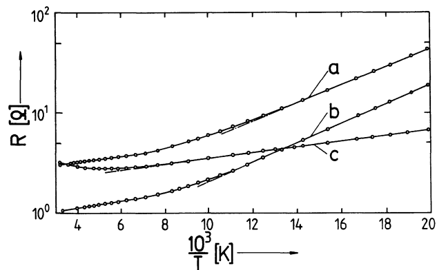
Fig. 3. — Electrical resistance as a function of inverse temperature of Fe 1+x Nb 3-x Se 10 (x = 0.32; 0.38) and of Cr 1.45 Nb 2.55 Se 10 between 300 and 50 K.
