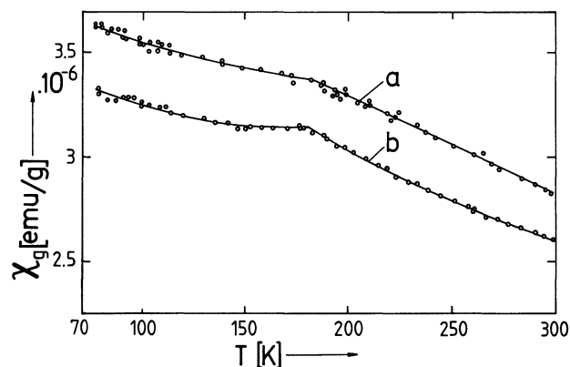
Fig. 7. — Temperature dependence of the magnetic susceptibility for Cr 1.45 Nb 2.55 Se 10 crystals. a) Magnetic field \perp b, c ; b) Magnetic field \parallel b .
