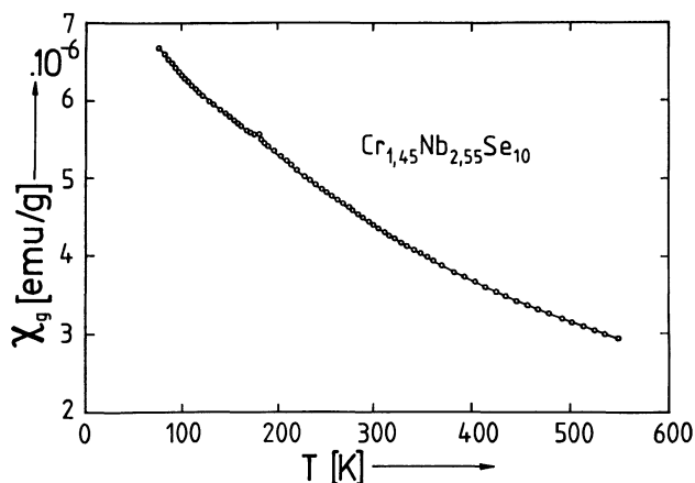
Fig. 6. — Temperature dependence of the magnetic susceptibility for Cr 1.45 Nb 2.55 Se 10 powder.
