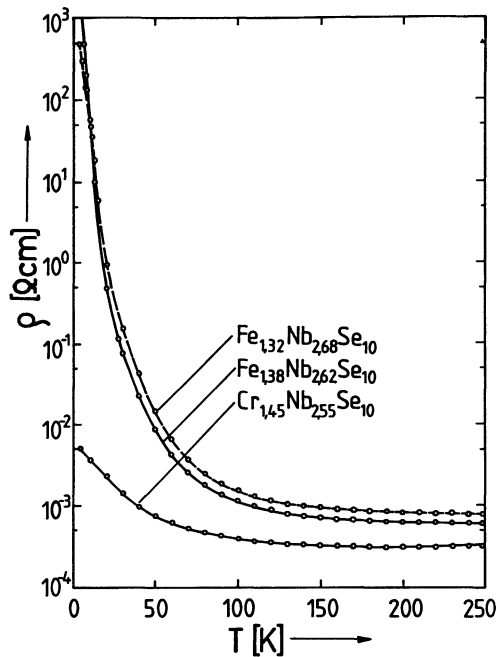
Fig. 1. — Temperature dependence of the resistivity of Fe 1+x Nb 3-x Se 10 (x = 0.32, 0.38) and of Cr 1.45 Nb 2.55 Se 10 .
