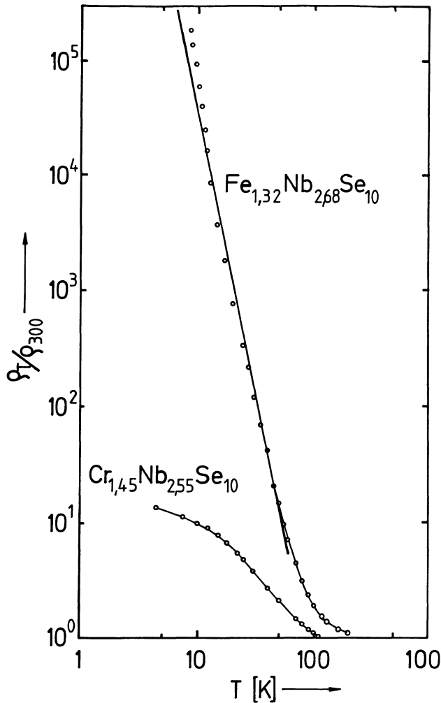
Fig. 4. — Resistivity relation \rho_T/\rho_{300} versus temperature for \text{Fe}_{1,32}\text{Nb}_{2,68}\text{Se}_{10} and \text{Cr}_{1,45}\text{Nb}_{2,55}\text{Se}_{10} plotted on log scales.
