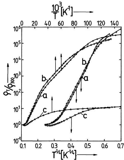
Fig. 2. — Resistivity relation \rho_T/\rho_{300} of Fe 1+x Nb 3-x Se 10 (x = 0.32; 0.38) and of Cr 1.45 Nb 2.55 Se 10 vs. T^{-1} (upper scale) and T^{-1/4} (lower scale) between 300 and 4.2 K. a) Fe 1.38 Nb 2.62 Se 10 , b) Fe 1.32 Nb 2.68 Se 10 , c) Cr 1.45 Nb 2.55 Se 10 .
