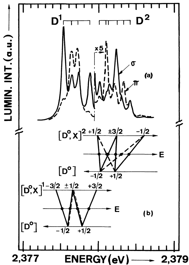
Fig. 3. — (a) Zeeman splittings of the D 1 and D 2 lines at a magnetic field of H = 3.5 T for H \parallel \langle 100 \rangle at T \approx 1.8 K for \sigma and \pi polarizations. (b) Corresponding schematic diagram showing Zeeman effects in the BE excited state [D^0, X]^2 and in the donor ground state [D^0] .
