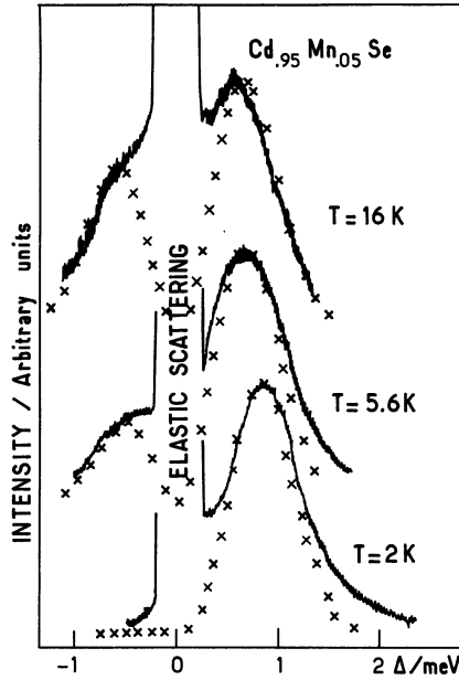
Fig. 1. — SFRS spectra in zero external field and for various temperatures, in Cd 0.95 Mn 0.05 Se. Exciting energy is 1.867 eV ( \lambda = 6637 Å). Theoretical curves (x) are generated from equations (4) and (15), with \sqrt{2} W_0 = 0.62 meV and T_{AF} = 0.6 K.
