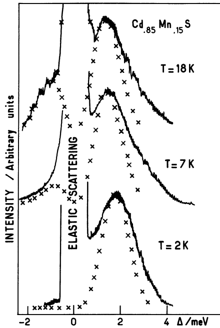
Fig. 2. — SFRS spectra in zero external field and for various temperatures, in Cd 0.85 Mn 0.15 S. Exciting energy is 2.540 eV ( \lambda = 4880 Å). Theoretical curves (x) are generated from equations (4) and (15), with \sqrt{2} W_0 = 1.2 meV and T_{AF} = 1.2 K.
