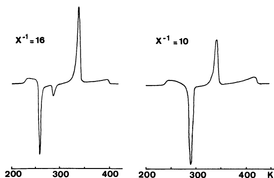
Fig. 2. — DSC traces for PEO(LiCF 3 SO 3 ) 1/10 and PEO(LiCF 3 SO 3 ) 1/16 obtained after heating at 450 K and cooling down at 320 K/min.
