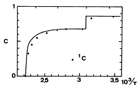
Fig. 3. — Fractions of protons 1 C belonging to the crystalline phase in PEO(LiCF 3 SO 3 ) 1/4 . The line represents 1 C DSC obtained from the phase diagram corrected by the factor \alpha defined in the text.
