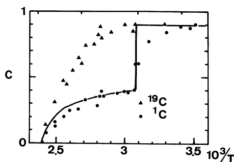
Fig. 4. — Fractions of protons 1 C (●) and fluorine 19 C (▲) belonging to the crystalline phase in PEO(LiCF 3 SO 3 ) 1/8 . The line represents 1 C DSC obtained from the phase diagram corrected by the factor \alpha defined in the text.
