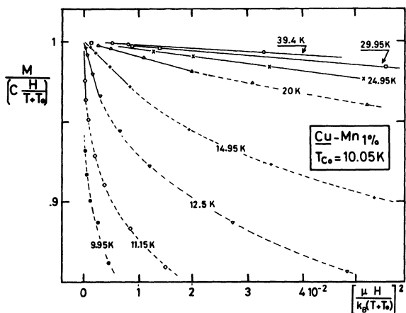
Fig. 5. — The same data as in figure 4 are represented in a M \left( \frac{CH}{T^*} \right)^{-1} vs. \left( \frac{\mu H}{kT^*} \right)^2 diagram. The slope of the initial straight line is the coefficient of (H/T^*)^3 in the development of the magnetization. It is seen to vary by orders of magnitude in our range of temperature.
