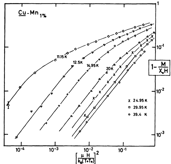
Fig. 13. — \text{Log}(1 - M/\chi_0 H) vs. \text{Log}\left(\frac{\mu H}{kT^*}\right)^2 . This diagram shows that an accuracy better than 10^{-3} on M/H is necessary in order to conclude on the temperature dependence of the H^3 term of the magnetization. Compare this plot with the figure 4 of reference 25.
