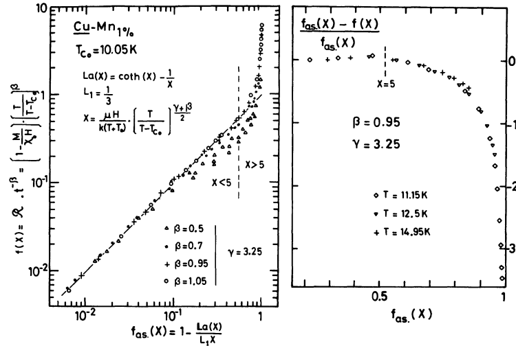
Fig. 10. — On the left hand side, \mathcal{R}t^{-\beta} from the experiments is compared to its theoretical value f_{as}(X) = 1 - \frac{La(X)}{L_1 X} (as derived from the high temperature regime X = 0 ) in a Log-Log plot for different values of \beta . Despite a relative insensitivity of our data to the values of \beta (for 0.5 < \beta < 1.05 ), we observe on this figure a degradation of the validity of the scaling and, at the same time, of the fit to the asymptotic expression if we try to decrease \beta below 0.7. It is in fact near T_c (for X > 5 where our asymptotic expression is no more valid) that we may hope to reach a more accurate determination of \beta . Further details are seen on the error curve -\frac{\mathcal{R}t^{-\beta} - f_{as}(X)}{f_{as}(X)} vs. f_{as}(X) which is shown on the right-hand side for \beta = 0.95 .
