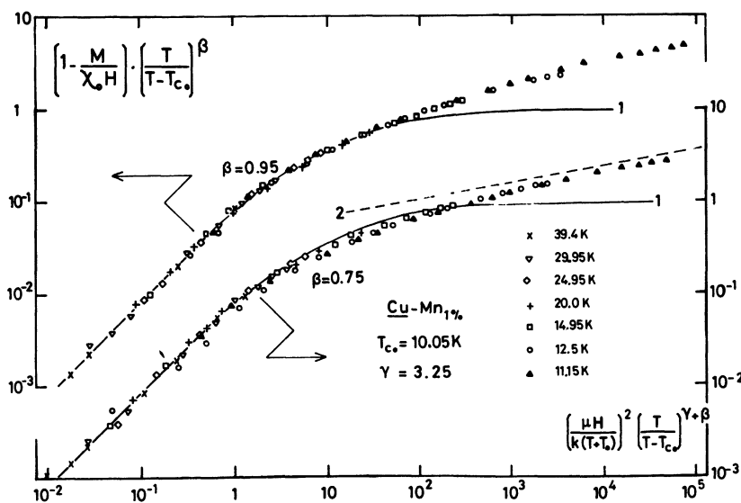
Fig. 9. — Universal plot of \left[1 - \frac{M}{\chi_0 H}\right] \left(\frac{T}{T - T_c}\right)^\beta vs. \left(\frac{\mu H}{kT^*}\right)^2 \left(\frac{T}{T - T_c}\right)^{\gamma+\beta} showing the success of the scaling argument for all our data points ( H up to 70 kOe, T up to 4 T_c ) with \gamma = 3.25 and \beta = 0.75 as deduced from the temperature dependence of a_3 and a_5 . The continuous curve 1 and the dashed curve 2 give the asymptotic behaviours predicted by equations 14 and 16 respectively. For \beta \approx 1 , we obtain a better fit to the expression 14 and an improved scaling.
