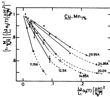
Fig. 6. — (1 - M/\chi_0 H) \left[ \frac{L_3 a_3}{L_1} \left( \frac{\mu H}{kT^*} \right)^2 \right]^{-1} vs. \frac{L_3}{L_1} a_3 \left( \frac{\mu H}{kT^*} \right)^2 . On this plot, the slope of the initial straight line is proportional to a_5 \cdot (L_3 a_3)^{-2} . The use of L_3 a_3 units allows us to present on a single figure data which vary by 6 orders of magnitude.
