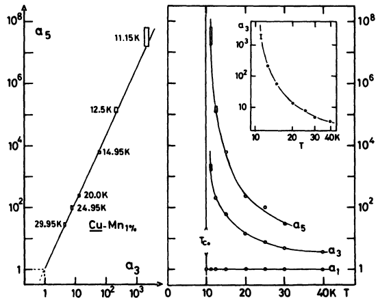
Fig. 7. — The coefficients a_1, a_3, a_5 involved in the series expansion of the magnetization in terms of x = \frac{\mu H}{kT^*}
