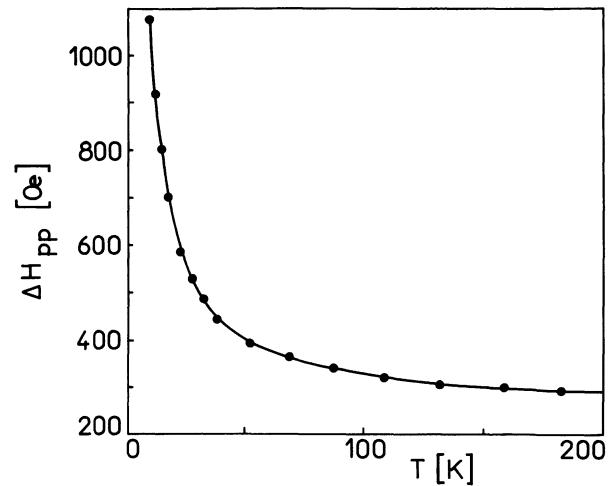
Fig. 6. — EPR peak-to-peak linewidth vs. temperature.
