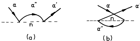
Fig. 1. — The two diagrams controlling the second order scaling of T_{\alpha\alpha'} . The dotted line denotes the impurity state n (inside the manifold \epsilon_0 ). The full line is the free electron propagator (diagonal in the index \alpha = (m, \sigma) ).
