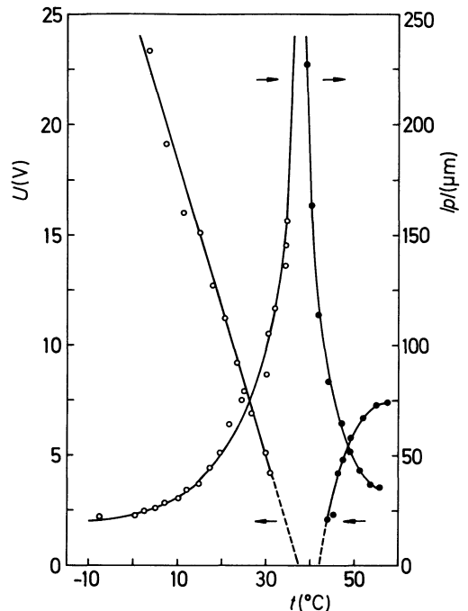
Fig. 4. — Threshold voltage measured with a cell thickness d of 125 \mu\text{m} and pitch versus temperature for an induced cholesteric mixture exhibiting a helix inversion at 39^\circ\text{C} (8.91 wt.-% CB 15 and 5.18 wt.-% S 811 in the nematic mixture E 8).
