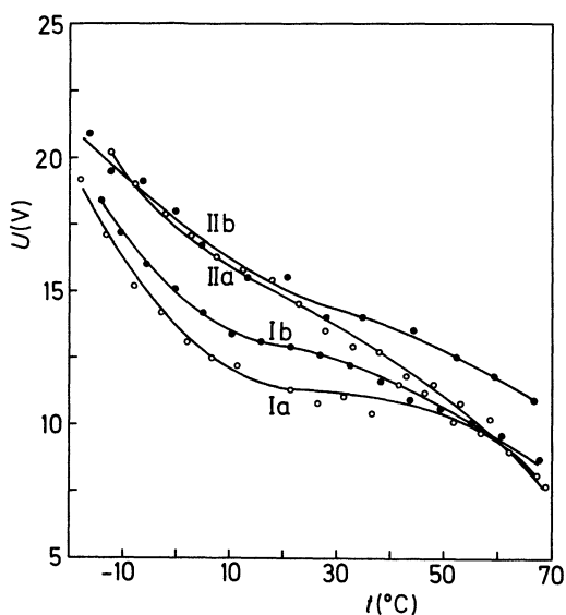
Fig. 2. — Temperature dependence of threshold voltage of the induced cholesteric phases obtained by the addition of one chiral compound. The cell thickness d was 23.5 \mu m .
