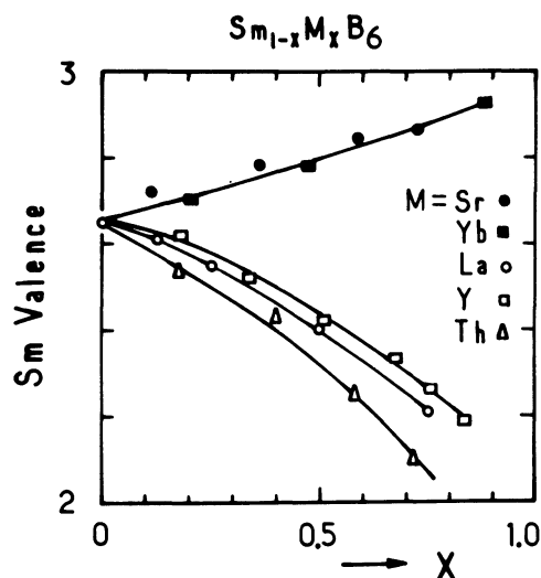
Fig. 6. — Average samarium valence determined from magnetic susceptibility measurements at 300 K in the \text{Sm}_{1-x}\text{M}_x\text{B}_6 systems ( \text{M} = \text{Yb}^{2+} , \text{Sr}^{2+} , \text{Y}^{3+} , \text{La}^{3+} , \text{Th}^{4+} ).
