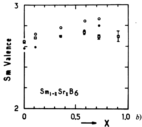
Fig. 8. — Average samarium valence at 300 K in the Sm_{1-x}M_xB_6 systems. Comparison of the results given by different methods. ● (black circles) X-ray absorption ; ○ (open circles) magnetic
