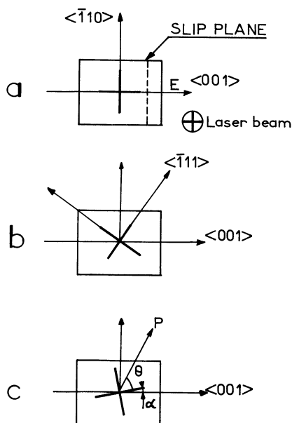
FIG. 1. — Orientation of the principal optical directions in a crystal of \text{NH}_4\text{Cl} for a light beam propagating along \langle 110 \rangle with stress birefringence produced by : a) Preexisting \{001\} slip bands or produced by an electric field E along \langle 001 \rangle ; b) Plastic deformation along \{111\} after the transition ; c) The simultaneous presence of these two effects. (P is the polarizer direction.)
