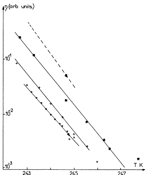
FIG. 8. — Exponential dependence of the residual long range order in the tail as a function of temperature above the mean transition temperature for different experiments : ○ Electro-optic effect (this work); + Second harmonic (square root of the intensity of diffracted second harmonic at its maximum), this work; * Second harmonic (square root of the intensity of diffracted second harmonic at its maximum), ref. [16]; -- Piezoelectric effect (ref. [11]). (The relative positions of these curves are arbitrary along the \eta axis.)
