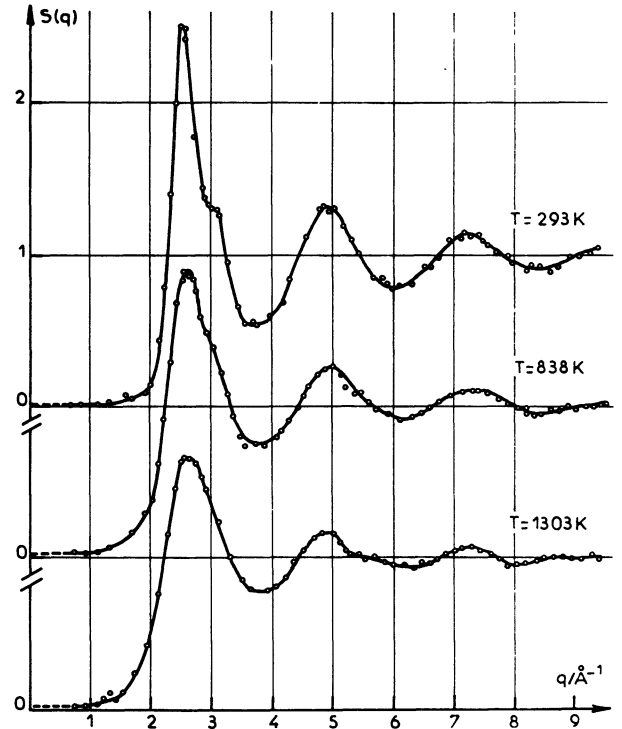
FIG. 2. — Structure factors obtained by neutron diffraction from liquid gallium at 293, 838 and 1 303 K.
