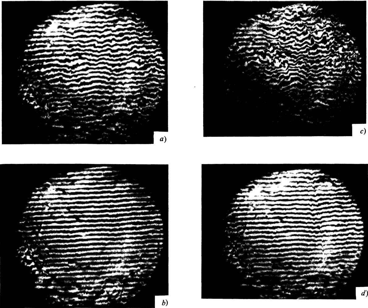
FIG. 2. — Interference-polarizing pictures of planar MBBA layer. Microscope — MPI-5, green light, layer thickness — 30 \mu\text{m} . With homogeneous orientation the lines are parallel. a) Zero voltage — the initial orientation is not ideal. b) High frequency a.c. voltage (10 V, 20 kHz) — the dielectric torque improves the planar orientation. c) d.c. voltage (1V) — deforming action. The deformation pattern is somewhat irregular. In the upper left corner a region with strong anchoring can be seen where there
