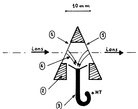
FIG. 1. — Start detector. 1) 10 \mu\text{g}/\text{cm}^2 carbon foils at a potential of 1 kV. 2) Prism supporting the foils. 3) Electron channel multiplier operating at 3 kV. 4) Trajectories for electrons ejected from the carbon foils during the passage of reaction products. The electrons are accelerated by the 1 kV potential between the foils and the collecting cone of the electron multiplier.
