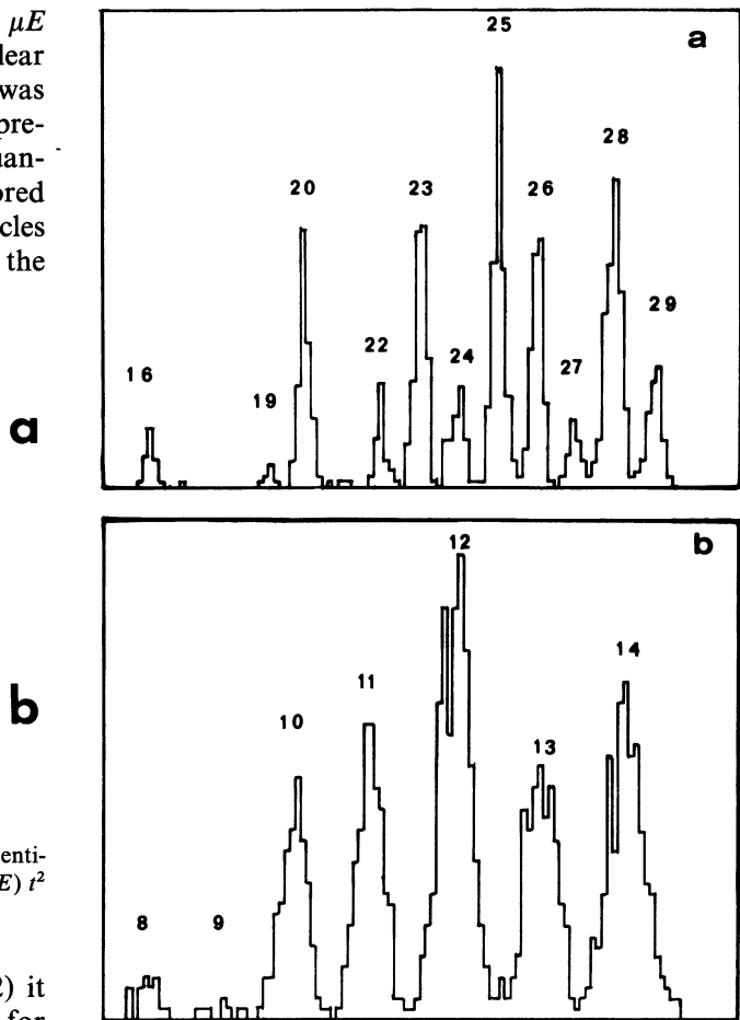
FIG. 3. — Typical spectrum of mass and charge identification at 6^\circ lab for v^2 corresponding to the average velocity of the recoiling compound nucleus ^{32}\text{S} .
