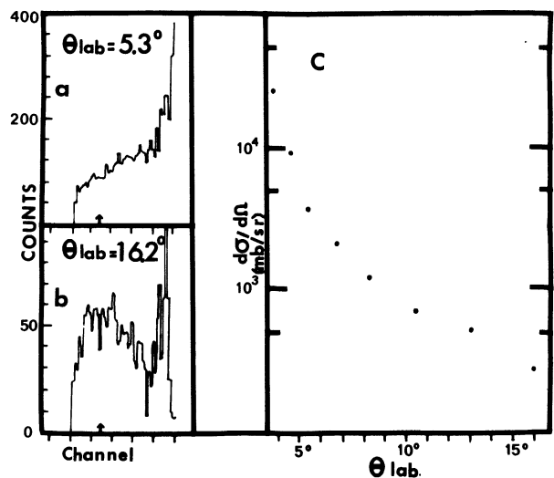
FIG. 4. — ^{20}\text{Ne} energy spectra (a, b) and angular distribution (c). The arrows in the energy spectra indicate the energy corresponding to the velocity of the recoiling ^{32}\text{S} nucleus.
