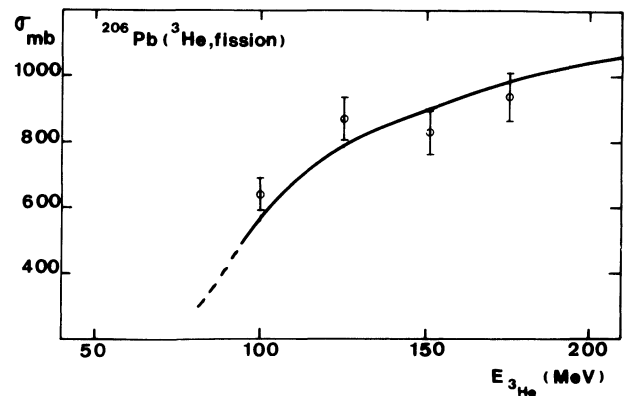
FIG. 7. — Excitation function for ^{206}\text{Pb}(^3\text{He}, \text{fission}) .
