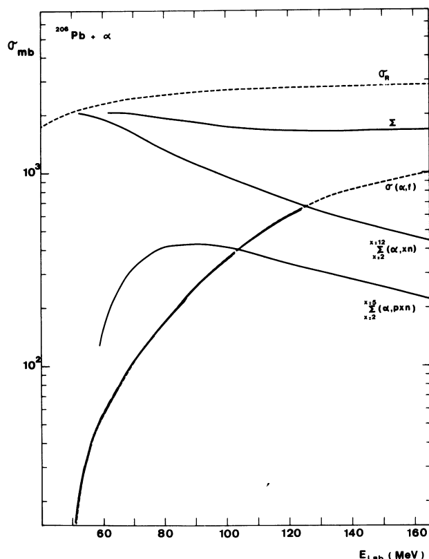
FIG. 10. — Contribution of different types of reactions to the ^{206}\text{Pb} + \alpha system.
