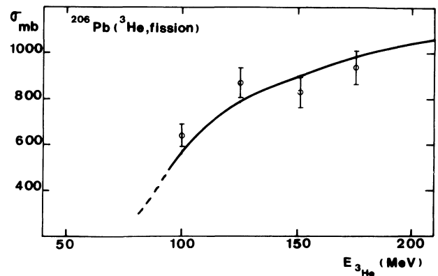
FIG. 7. — Excitation function for ^{206}\text{Pb}(^3\text{He}, \text{fission}) .
