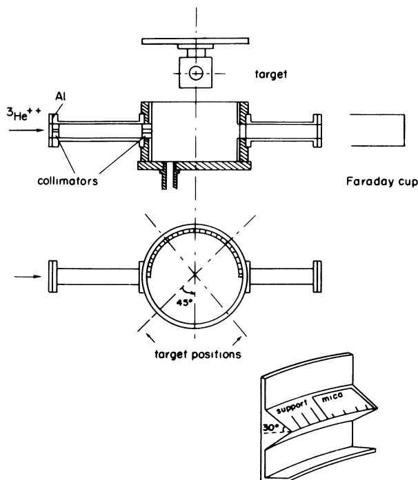
FIG. 1. — Schematic diagram of irradiation chamber and mica foil supports.
