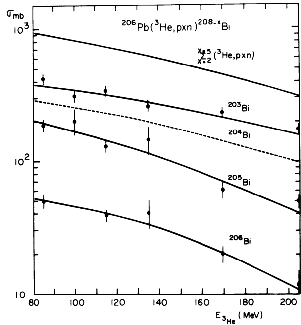
FIG. 5. — Excitation functions for ^{206}\text{Pb}(^3\text{He}, pxn) reactions for x = 2-5 . Curve for x = 4 is estimated.
