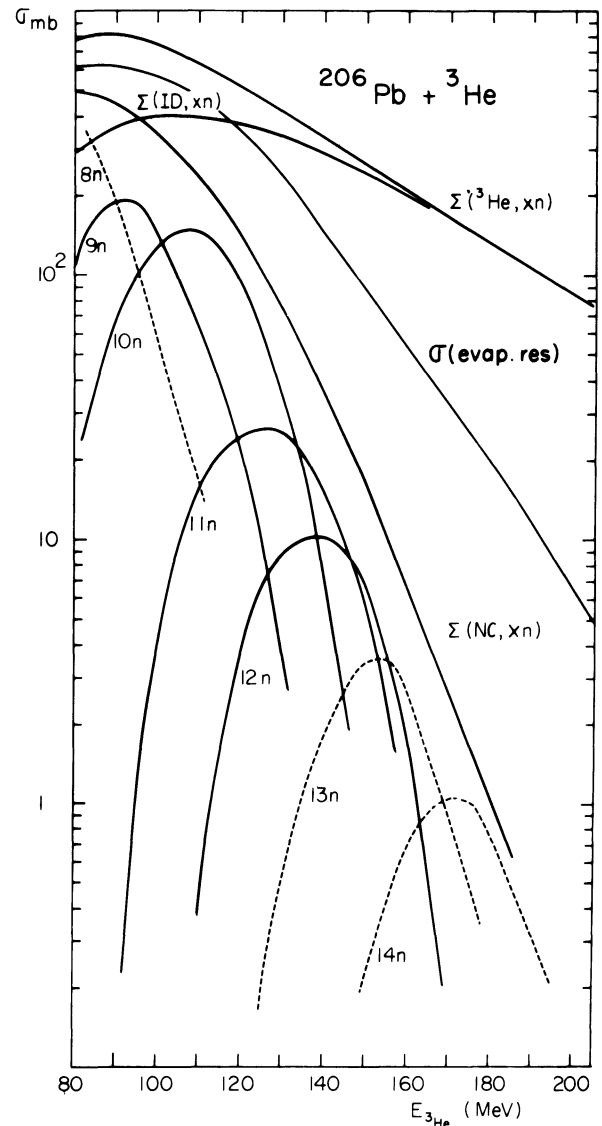
FIG. 9. — Contribution of compound nuclear mechanism to ( {}^3\text{He}, xn ) reactions. Curves for x = 13 and 14 are estimated.
