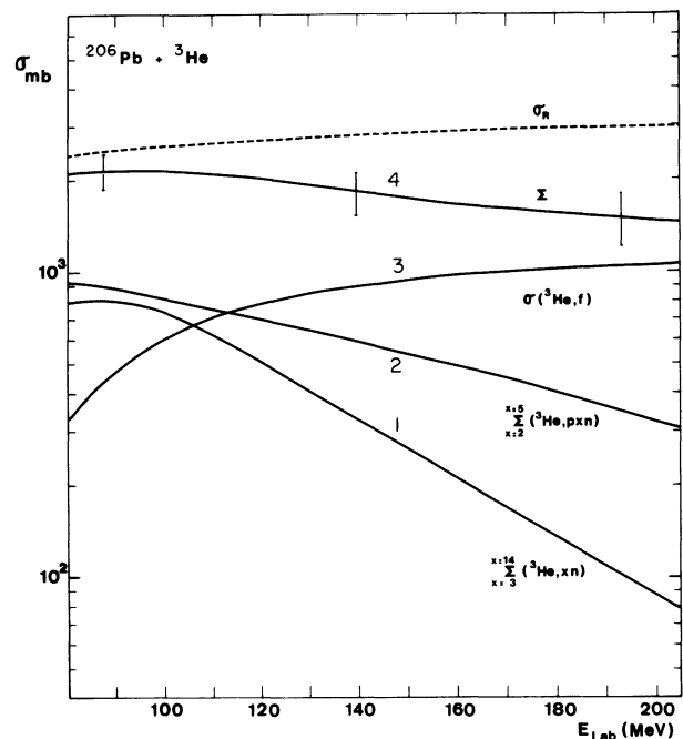
FIG. 8. — Contribution of different types of reactions to the {}^{206}\text{Pb} + {}^3\text{He} system.
