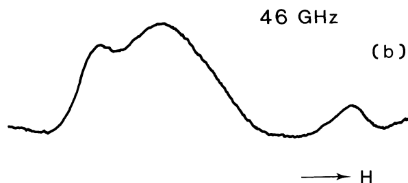
FIG. 1b. — ESR spectrum at 1.5 K, 46 GHz, and the microwave power level of -6 \text{ dB} for sample M4 ( N_D = 3.1 \times 10^{17} \text{ cm}^{-3} ).
