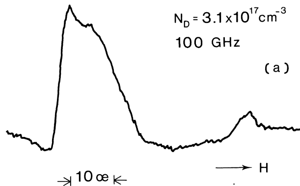
FIG. 1a. — Typical trace of ESR spectrum at 1.4 K, 100 GHz and the microwave power level of -3 \text{ dB} for sample M4 ( N_D = 3.1 \times 10^{17} \text{ cm}^{-3} ).
