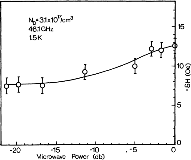
FIG. 2. — Peak shift, \delta H , as a function of microwave power at 1.5 K and 46 GHz for sample M4 ( N = 3.1 \times 10^{17} \text{ cm}^{-3} ) (after ref. [6]).
