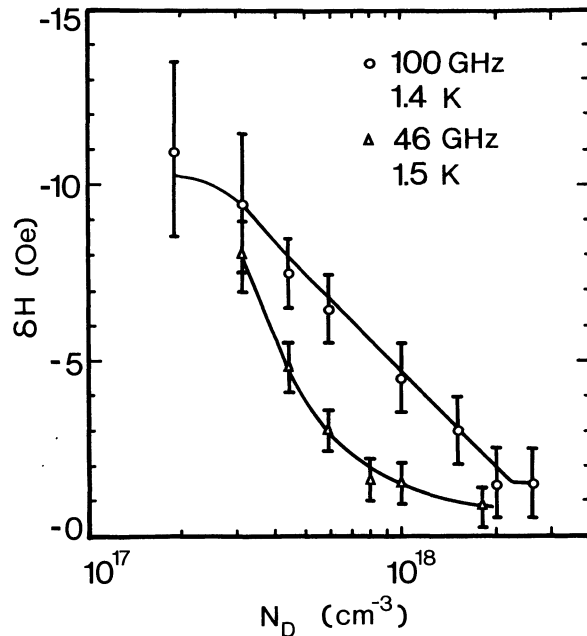
FIG. 3. — Peak shift, \delta H , as a function of donor concentration, N_D , at 1.4 K and 100 GHz and also at 1.5 K and 46 GHz, in the low power limit.
