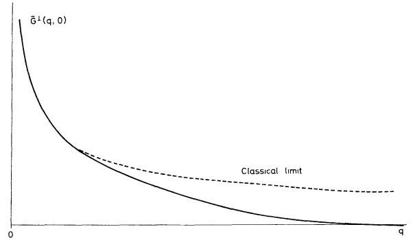
FIG. 7. — Fourier transform of figure 6 at t = 0 .
