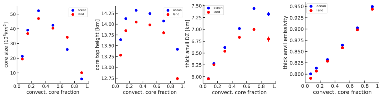
Figure 8: MCS properties as function of their life cycle stage, given by fraction of convective core area within the system (1 corresponds to developing phase, with no anvil and 0.1 to dissipating stage): size and top height of the convective cores, vertical extent and emissivity of the thick anvils (emissivity > 0.5). Statistics combines observations at 1:30AM and 1:30PM, for 2008-2018.
