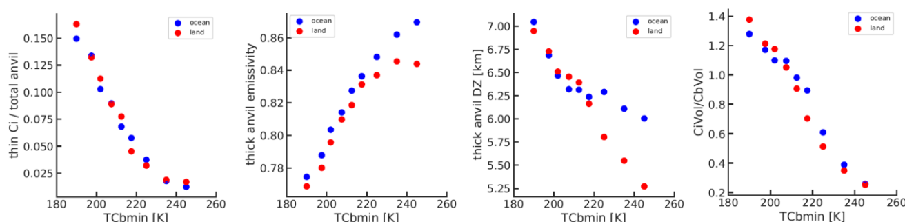
Figure 9: Mature MCS system properties as function of their convective depth, given by the minimum temperature within the convective cores: ratio of areas with thin cirrus over total anvil, thick anvil emissivity and ratio of strong rain area over rainy area (right) within mature convective systems as a function of convective depth, given by decreasing minimum temperature within the convective cores. The convective cores are defined by cloud emissivity > 0.93, fraction of Cb within grid cell > 0.2 and DZ/Z top > 0.6. Different thresholds on the fraction of rain per grid cell to be included into the areas are compared. The condition on strong rain also includes the condition that at least 50 of the grid cells are covered by any rain. Statistics combines observations at 1:30AM and 1:30PM, for 2008-2018.
