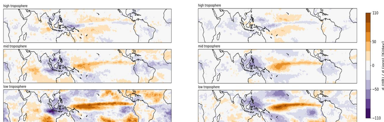
Figure 13: Change in radiative heating rates with respect to deseasonalized I_{org} computed from convective areas defined by grid cells with rain indicator > 2 (left) and by grid cells with T_{cld} < 230 K and \epsilon_{cld} > 0.95 (right). The troposphere is divided into three layers: upper troposphere (100–200 hPa), mid troposphere (200–600 hPa), and low troposphere (600–900 hPa). Monthly statistics from 2008 to 2018.
