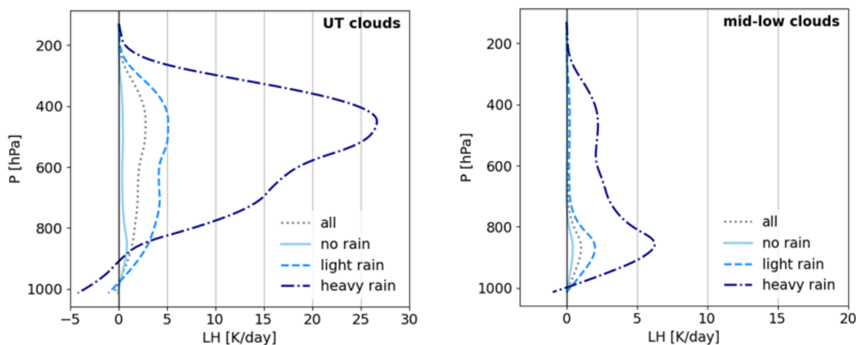
Figure 5: Average latent heating profiles derived from TRMM (Shige et al., 2009) produced by UT clouds (left) and by mid- and low-level clouds (right) identified by AIRS, at the local time of 1:30 AM. In addition to the tropical mean are shown means of non-precipitating, lightly precipitating and heavily precipitating clouds. These precipitation conditions are given by the rain rate indicator classification derived from CloudSat and AIRS-ERA Interim machine learning. Statistics of collocated TRMM-AIRS in the period 2008-2013.
