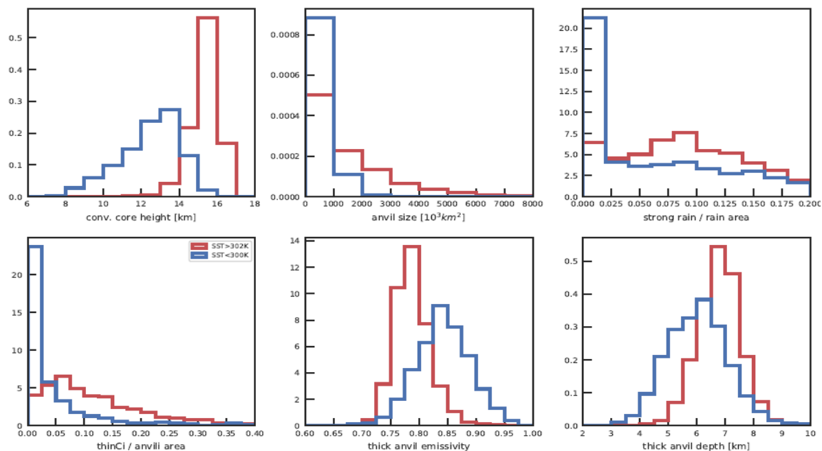
Figure 10: Normalized frequency distributions of mature MCS system properties over the 30% warmest and coolest tropical ocean regions. Top panel rom left to right: height of convective cores, size of anvils, and ratio of areas with strong over total precipitation; bottom panel from left to right: ratio of areas with thin cirrus over total anvil, thick anvil emissivity, and thick anvil vertical extent. Statistics combines observations at 1:30AM and 1:30PM, for 2008-2018.
