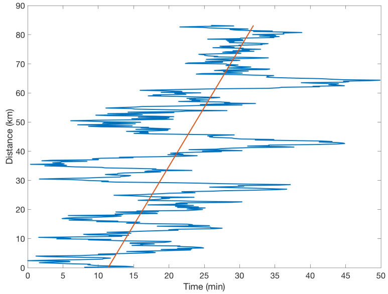
Figure 7. Temporal phase evolution of the 150 min wave extracted from the East-West keogram, the red line is the linear fit.
