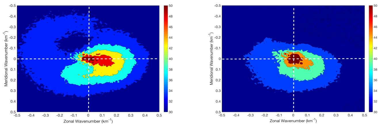
Figure 16. Left : Unambiguous horizontal wavenumber spectra (UHWS) from the OH images of the first part of the night, before midnight. Right : UHWS of the second part of the night, after midnight. The color bar in the 2-D spectrums is in logarithmic scale and representing the square of the magnitude ( \text{cyc}/\text{m} ) 2 . White dashed lines shows the position of the zero wavenumbers.
