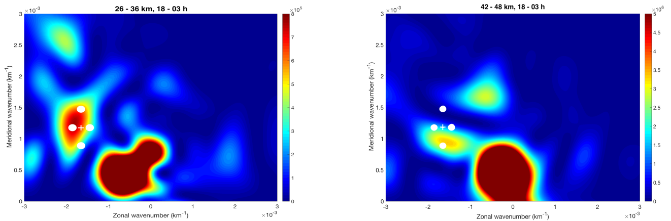
Figure 8. Left : Average 2D Fourier spectrum of ERA 5 temperature fields for the altitude range 26-36 km (left) and 42-48 km (right) for the time range [18 p.m. 03 a.m.]. The white cross represents the wavenumbers estimated using the OH keograms. The cross are the estimated errors on the wavenumbers, calculated directly from the error on the slope of the linear fit (Figure 7).
