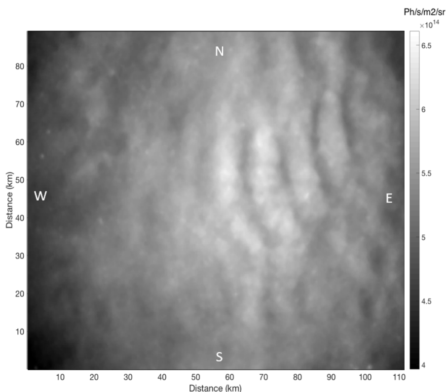
Figure 2. Corrected image of the OH radiation at altitude 87 km acquired during the night of the 12th-13th December 2017 [20]. The radiance scale is in ph/s/m 2 /sr. North is at the top of the image, west on the left.
