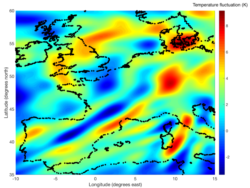
Figure 3. Horizontal field of anomaly temperature extracted from ERA5 re-analysis during the night of the December 12-13, 2017 at 18 h UT over Western Europe around 49 km altitude.
