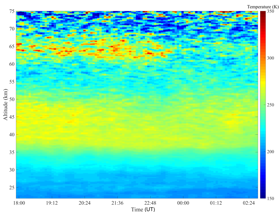
Figure 1. 2D Temperature profile measured by the OHP Rayleigh lidar during the night of the December 12-13, 2017
