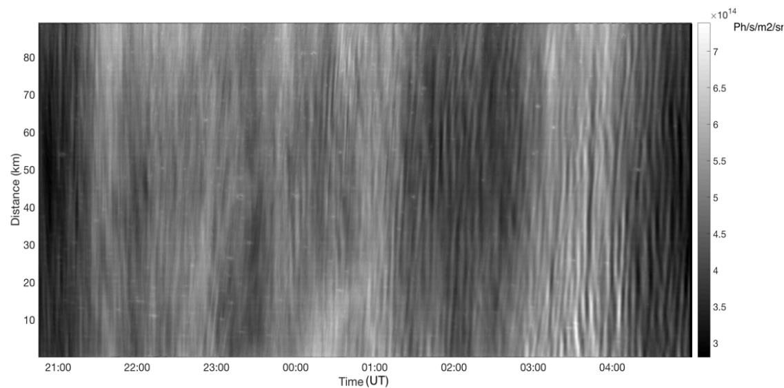
Figure 5. North-South keogram for the night of December 12-13, 2017 composed from a series of OH images. The grey scale is in \text{ph/s/m}^2/\text{sr} .
