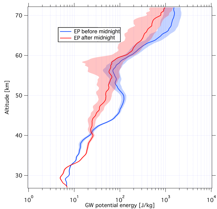
Figure 11. Evolution of potential energy with altitude before midnight (blue curve) and afterwards (red curve). The shaded areas are the associated errors [11].
