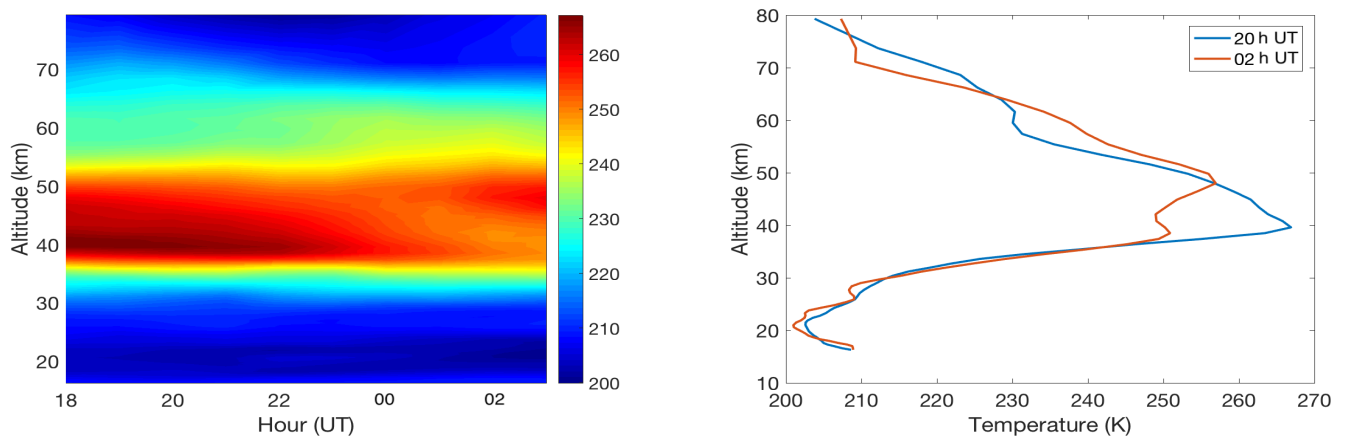
Figure 10. Left : 2D temperature profile during the night of the December 12, 2017 from the ERA5 data. Right : Temperature profile at 20 h UT in blue and 02 h UT in red from the ERA5 data.
