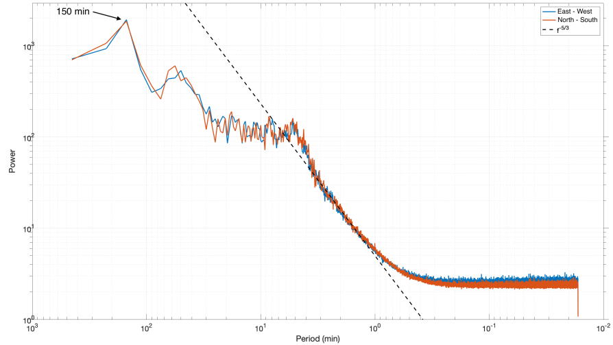
Figure 6. Mean Fourier spectrum of the entire night for the two keograms. The black dash line is the -5/3 power law. L is the radiance unit measured on the OH images ( \text{ph/s/m}^2/\text{sr} ).
