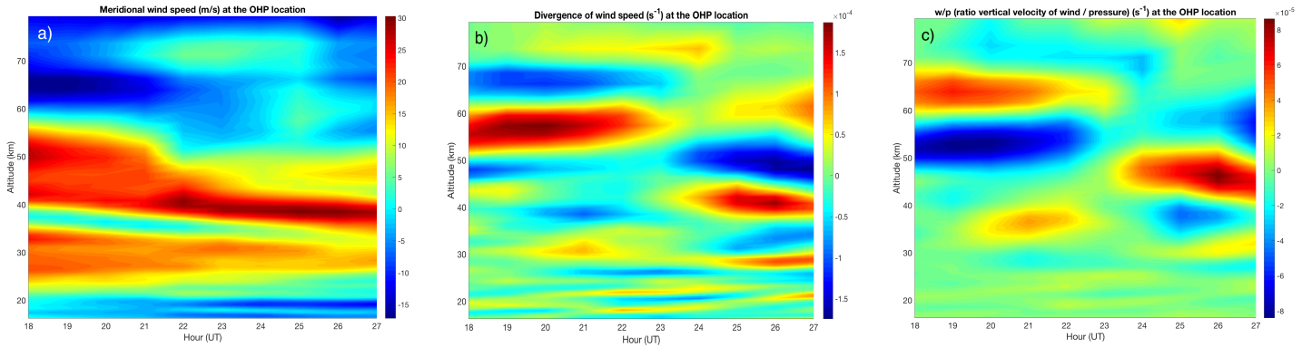
Figure 13. a) Meridional wind speed in \text{m}\cdot\text{s}^{-1} from ERA5 data. b) Divergence of wind speed in \text{s}^{-1} from ERA5 data. c) Vertical wind speed (in \text{Pa}\cdot\text{s}^{-1} divided by pressure (in Pa))
