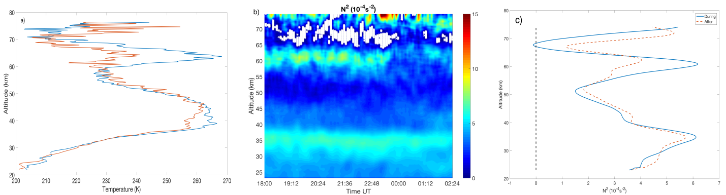
Figure 9. a) Rayleigh lidar temperature profiles. The blue curve represents the average temperature for each altitude before midnight and the red curve is the average temperature after midnight [20]. b) Square Brunt-Väisälä frequency profile during the night of December 12, 2017 at the Haute-Provence observatory. White dots show negative values. c) Mean Square Brunt-Väisälä frequency profile before midnight in blue and after midnight in red. The 0 value is indicated by the dotted black vertical line.
