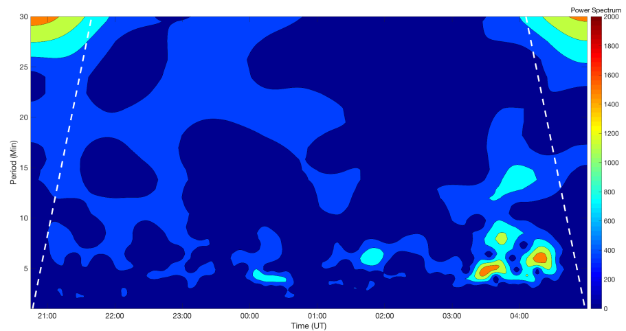
Figure 14. Contour plot of the wavelet analysis of the temporal OH radiance profile. The white dashed lines represent the cone of influence which delimits the real periods of the discontinuities.
