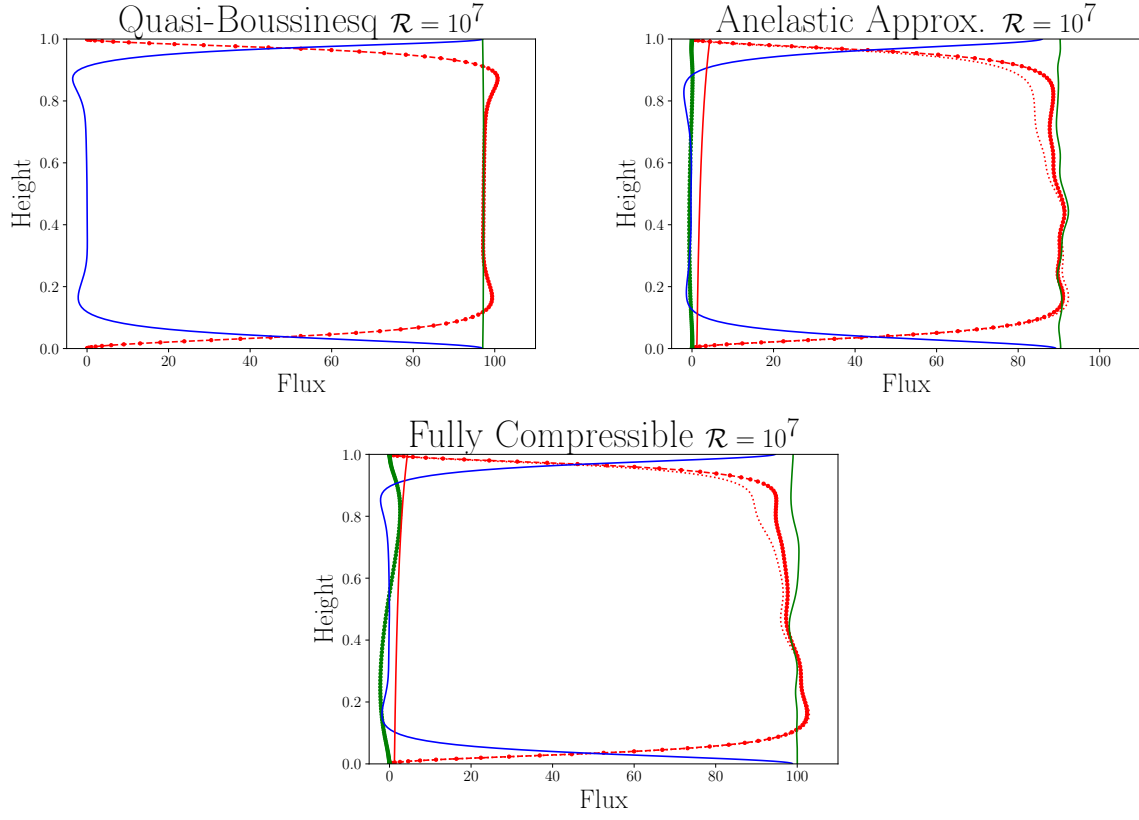
Figure 19: Same as Figure 11 for \mathcal{R} = 10^7
