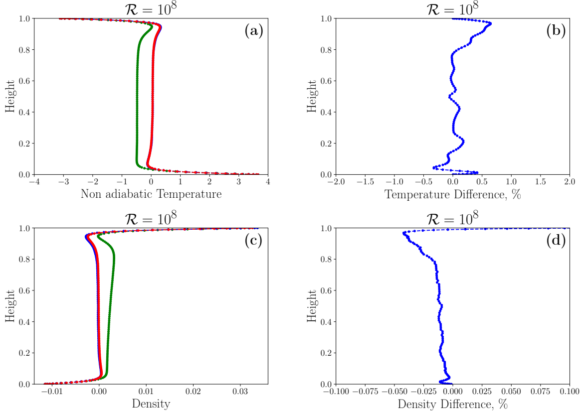
Figure 10: Same as Figure 9 but for \mathcal{R} = 10^8 . The decrease of thermal expansivity with depth thickens the bottom thermal boundary particularly in the QB case and also decreases the bulk temperature and increases the density (green). The FC (red) and AA (blue) cases are difficult to distinguish except maybe below the top boundary layer where the AA predicts slightly hotter and denser conditions. We do not plot the differences between QB and FC curves as their amplitudes are very large.
