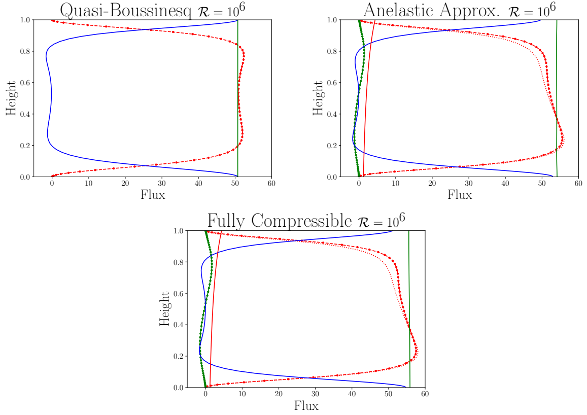
Figure 17: Different components of the heat flow profile across the convective layer for \mathcal{R} = 10^6 : for the QB case conduction (blue) and heat advection (red, dotted), for the AA and FC cases, we plot the conduction along the adiabat (red solid), and along the non adiabatic temperature profile (blue), the work flow (green, dotted), the advection of enthalpy (red, dotted) is larger than when the enthalpy is identified with the temperature.
