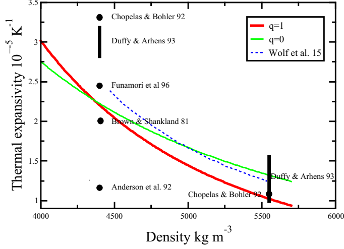
Figure 3: Thermal expansivity \alpha_a as a function of density in the Earth mantle using the parameters of Figure 1. The predictions are with q = 1 (solid red) and q = 0 (green). Various experimental observations with conditions appropriate for the top of the lower mantle or for the CMB are indicated by dots or vertical ranges.
