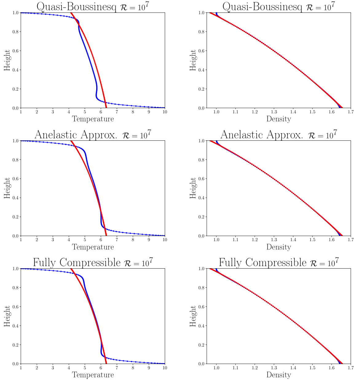
Figure 18: Quasi-Boussinesq and Anelastic approximations, Fully Compressible case. Mean temperature (left column) and density (right column) profiles for \mathcal{R} = 10^7 .
