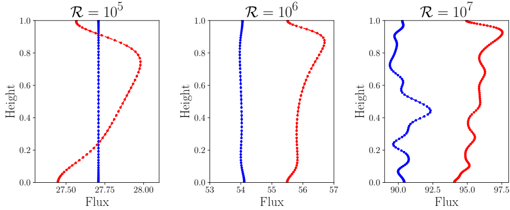
Figure 13: Heat flow profiles. Notice the small range of the horizontal scales. The classical anelastic equations (40) where the entropy is only related to temperature (ALA) and where the heat capacity ratio C_P/C_V is approximated as uniform leads to the heat flow depicted with red lines. Our formalism when the heat equation is (39c), leads to the predictions in blue. The inconsistency in the thermodynamics leads to a non-uniform heat flux increasing with height in the convective region and a surface heat flow overestimated by \approx 4\% at large \mathcal{R} number.
