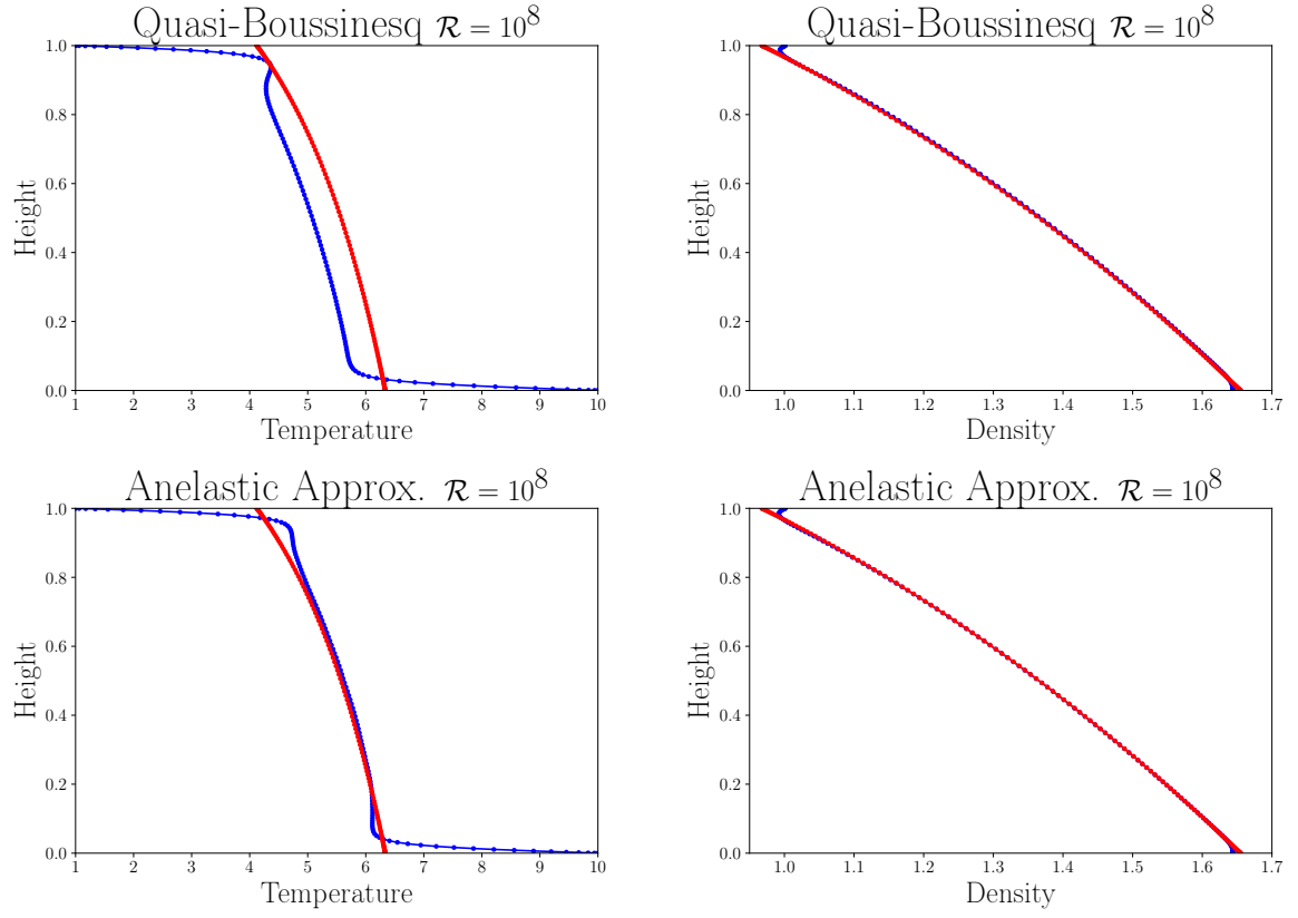
Figure 20: Quasi-Boussinesq and Anelastic approximations. Mean temperature (left column) and density (right column) profiles for \mathcal{R} = 10^8 .
