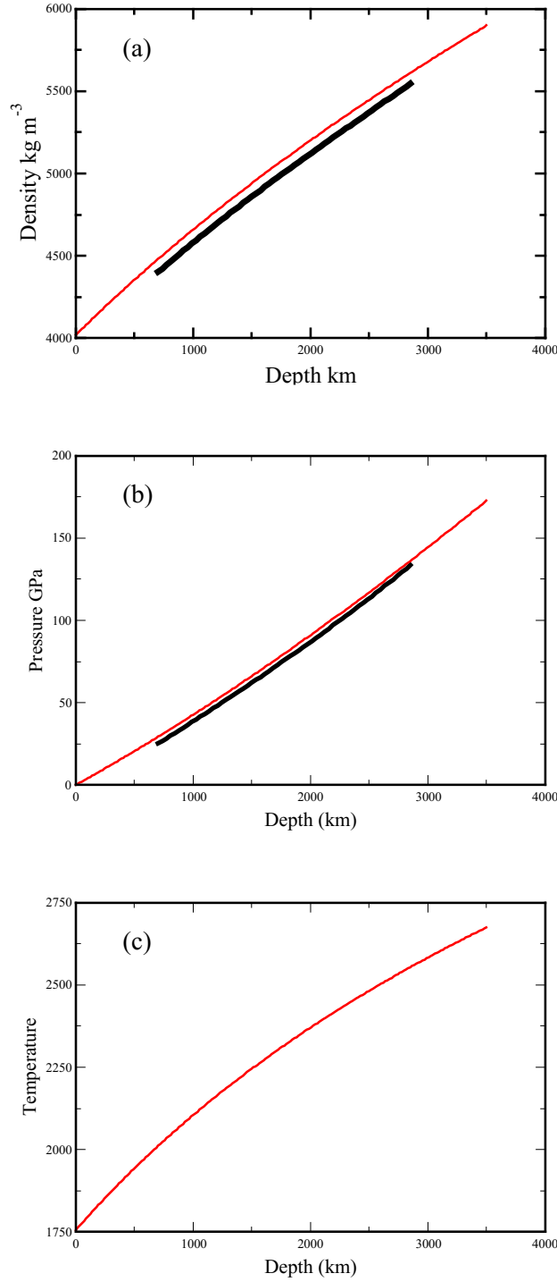
Figure 4: Adiabatic density (a), pressure (b) and temperature (c) as a function of depth using for the EoS the numerical values obtained by fitting the Earth lower mantle and assuming C_P = C_V . The density and pressure of PREM are shown in black. Since this model assumes a unique EoS for the upper and lower mantle, using values of Figure 1 (red line) fitted to the lower mantle and disregarding the different phases of the upper mantle, the predictions have a higher density and consequently, a higher pressure than PREM.
