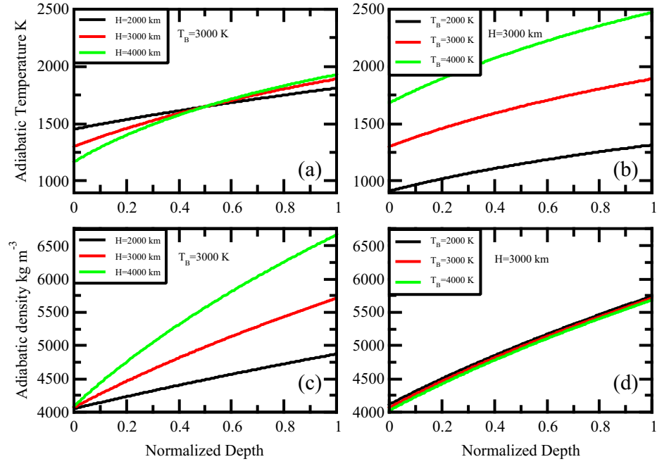
Figure 5: Possible density (using (14), bottom panels c and d) and temperature (top panels a and b) adiabatic profiles in various planets. In the left column, the mantle thickness is increased with a constant bottom temperature. Gravity scales with the mantle thickness. In the right column, the temperature is increased at constant mantle thickness. The Earth conditions are roughly similar to the intermediate case depicted in red.
