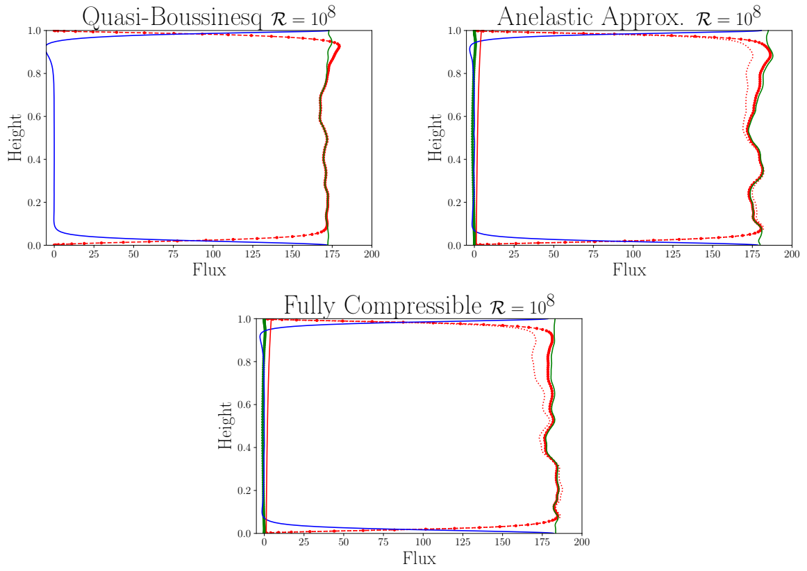
Figure 12: Similar to Figure 11 but for \mathcal{R} = 10^8 . The convection is short wavelength and very vigorous and it becomes more difficult to get accurate statistical values. The total heat flow (green lines) is reasonably uniform.
