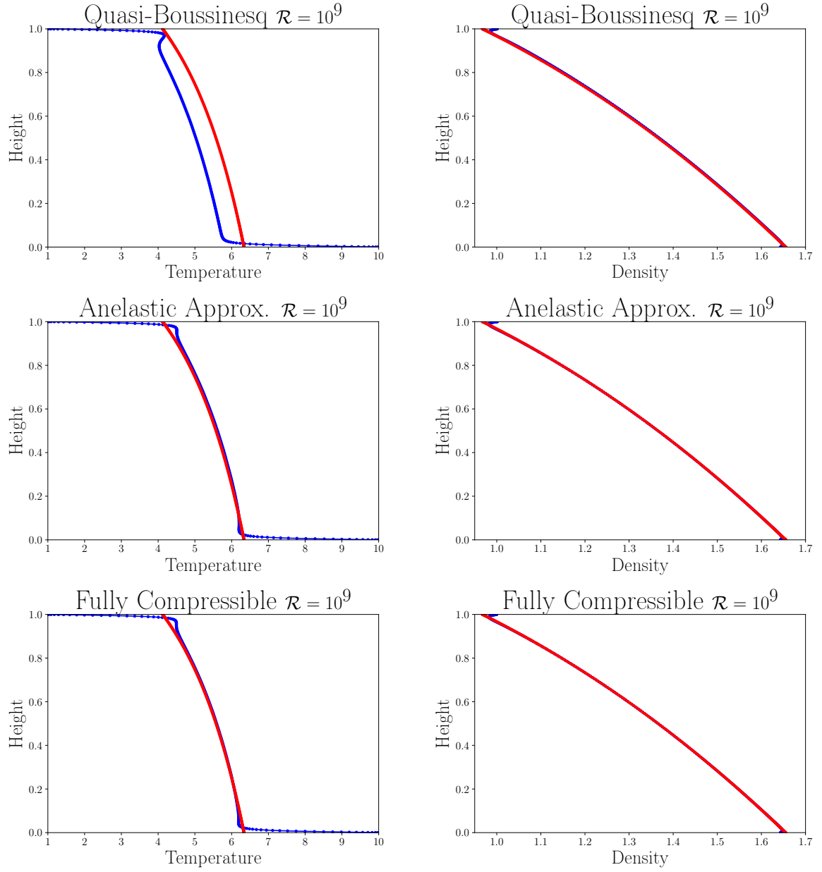
Figure 21: Quasi-Boussinesq and Anelastic approximations, Fully Compressible case. Mean temperature (left column) and density (right column) profiles for \mathcal{R} = 10^9 .
