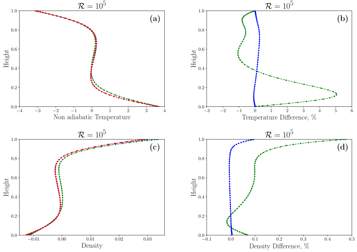
Figure 9: On the left column mean temperature (top) and density (bottom) profiles minus the adiabatic contribution are depicted for the FC (red), AA (blue) and QB (green) cases for \mathcal{R} = 10^5 . The different profiles being close together, we plot in the right column (b and d) the differences between the approximated set of equations and the exact result (i.e., (T_{AA} - T_{FC})/T_a in blue, (T_{QB} - T_{FC})/T_a in green), in percentage of the adiabatic temperature or density (panels c and d) expected at the same depth.
