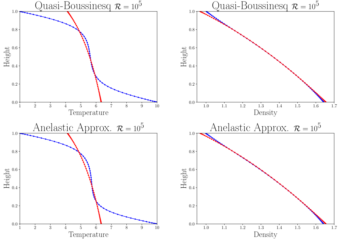
Figure 15: Quasi-Boussinesq and Anelastic approximations. Mean temperature (left column) and density (right column) profiles for \mathcal{R} = 10^5 .
