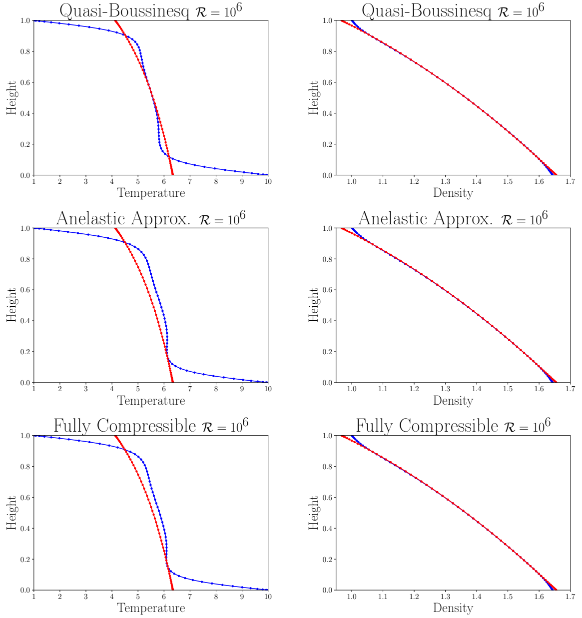
Figure 16: Quasi-Boussinesq and Anelastic approximations, Fully Compressible case. Mean temperature (left column) and density (right column) profiles for \mathcal{R} = 10^6 .
