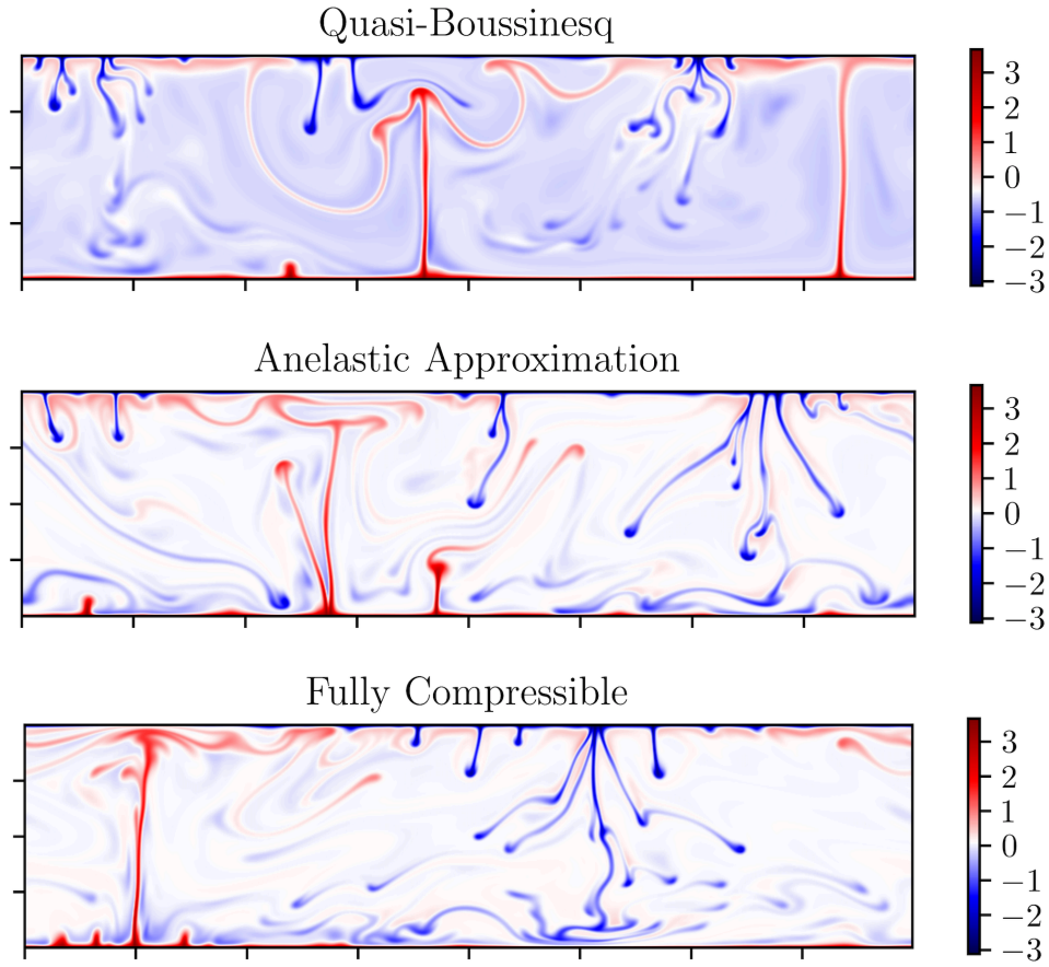
Figure 7: Snapshots of the non-adiabatic temperature field at \mathcal{R} = 10^9 using the QB, AA and FC approximations. The temperature color scales are slightly different in the three cases but over the same imposed non-adiabatic range. The QB temperature is clearly lower than in both other cases.
