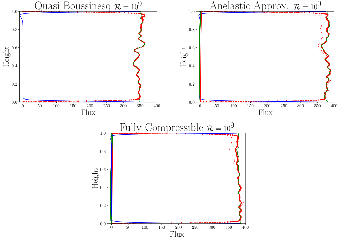
Figure 22: Same as Figure 19 for \mathcal{R} = 10^9
