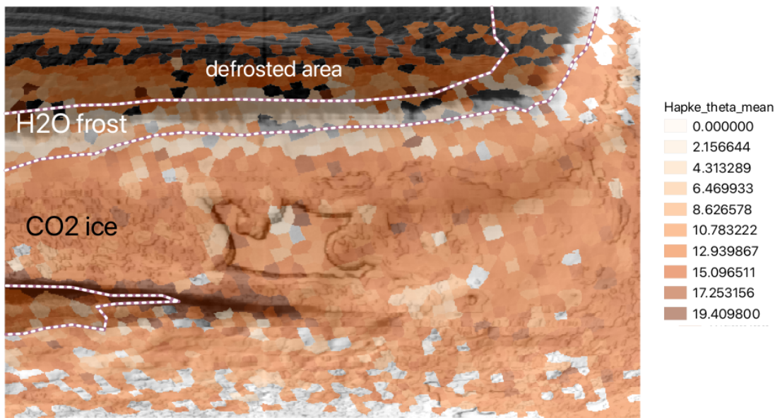
Figure 2: Mars South Pole dataset. Parameter \bar{\theta} averaged over spectral dimension.
