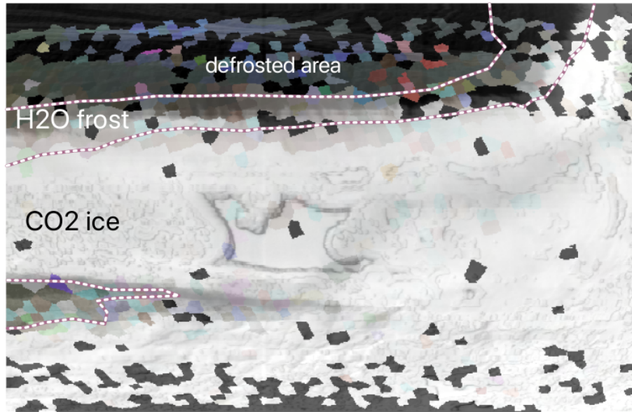
Figure 1: Mars South Pole dataset. Parameter \omega in synthetic colors coding 3 wavelengths.
