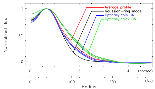
Fig. 3. Azimuthally averaged radial profiles of the integrated flux for the 7 hyperfine (hf) components of C^{14}N , four of which are optically thin, the remaining three being optically thick (Fig. 2). The average of the 7 hf components is shown in red. The black line shows the result of a sharp inner-ring model plus Gaussian decrease outwards, convolved by the synthesized beam. The unconvolved ring has a radius of 0.7'' or 42 AU, and a full-width at half-maximum of 54 AU (at a distance of 59.5 \pm 0.9 pc).
