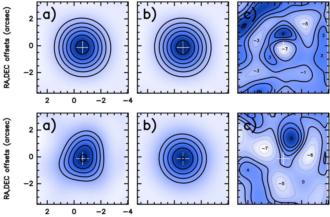
Fig. C.2. Results of the uv -plane analysis (see the text for details) for C^{14}N (top) and C^{15}N (bottom). On each row, panels a) and b) show the dirty image and the fitted Gaussian disk (Jy/beam), and panel c) shows the residuals (in mJy/beam). For C^{14}N , contours in panels a) and b) are 0.1 to 0.7 by 0.1 Jy/beam, and for C^{15}N from 0.02 to 0.07 by 0.01 Jy/beam. Values of local extrema are indicated in the residuals. The C^{15}N fit assumes the Gaussian disk from C^{14}N . The results are summarized in Table 1.
