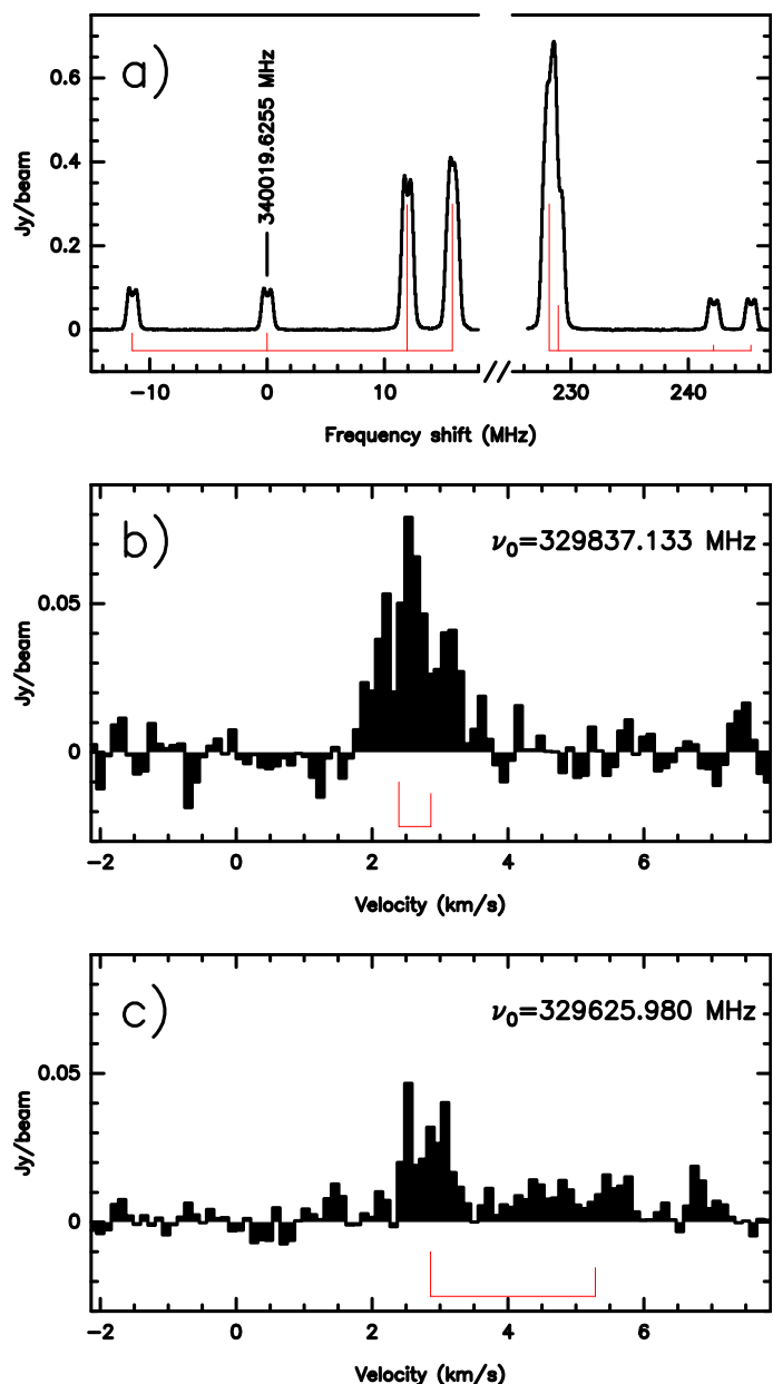
Fig. 1. Spectra, averaged within the dashed circle in Fig. 2, of the entire C 14 N (a) and of the two sets of hyperfine lines of C 15 N (b) and (c). The hyperfine splitting and relative strengths of the hf components are indicated below the spectra.
