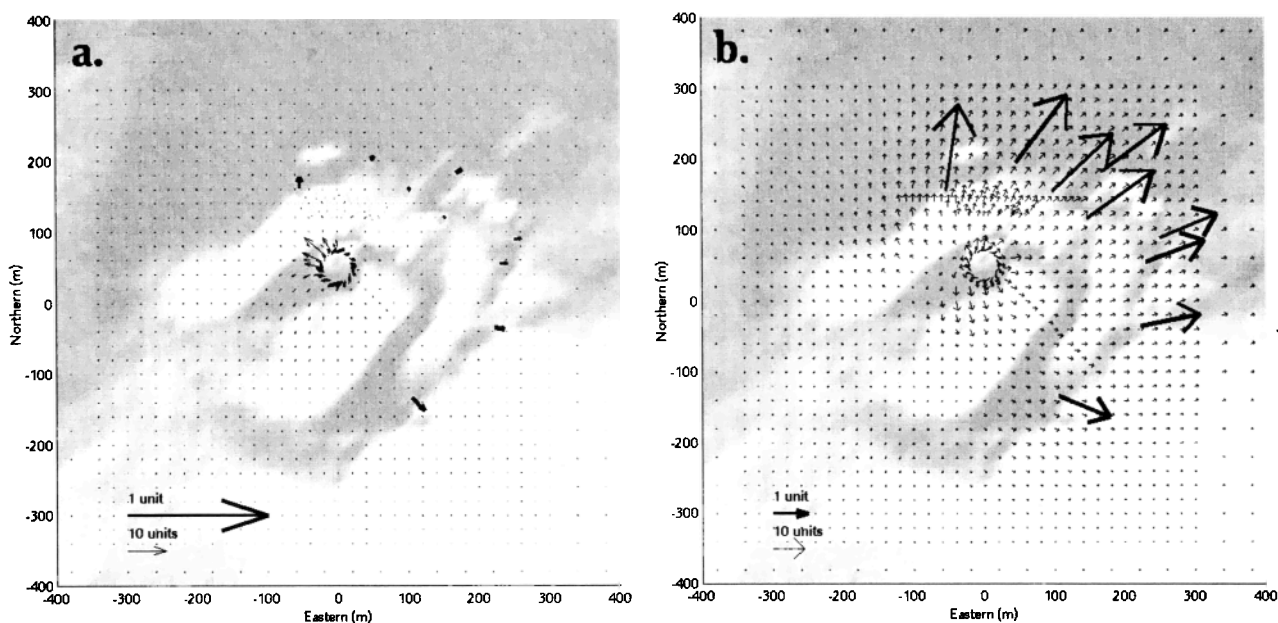
Figure 11. Displacement field computed without fracture in the medium. (a) Pressure source. (b) Wall shear stress source. Thick arrows stand for blowup displacements at GPS benchmarks position (different scale).
