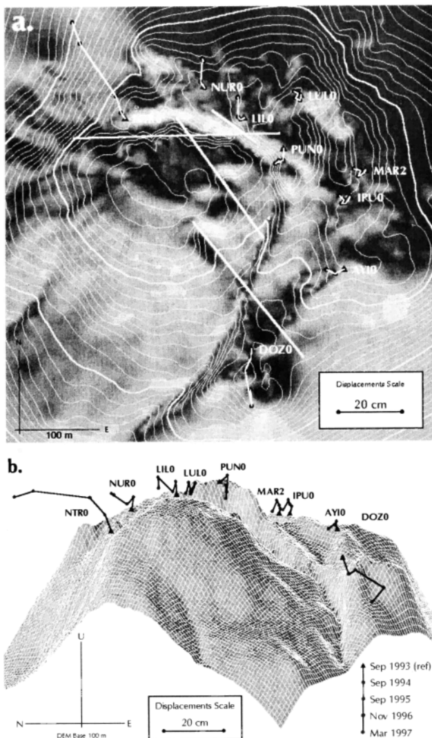
Figure 6. Cumulated displacements of GPS points from 1993 to 1997 and 1993 summit map. (a) horizontal view; (b) perspective view in a vertical plan (azimuth N145° E, elevation 0°), such that vertical displacements scale is respected.
