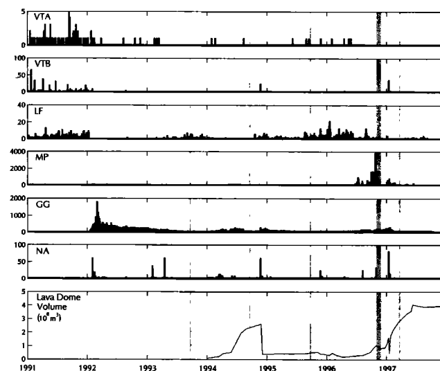
Figure 3. Seismic activity (number of events per day) and lava dome volume estimation from 1991 to 1997 (data from Ratdomopurbo and Suharno [1997]). VTA, deep volcano-tectonic (depth > 2 km); VTB, shallow volcano-tectonic (depth < 1.5 km); LF, low frequency (1.5 Hz); MP, multiphase; GG, “guguran” associated with rock avalanches; NA, nuées ardentes. Gray lines represent time of GPS campaigns.
