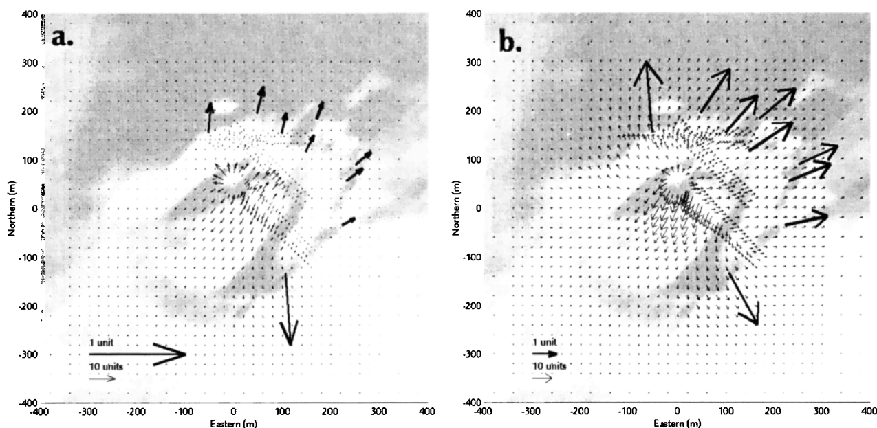
Figure 12. Displacement field computed with three fractures in the structure. (a) Pressure source. (b) Wall shear stress source. Thick arrows stand for blowup displacements at GPS benchmarks position (different scale).
