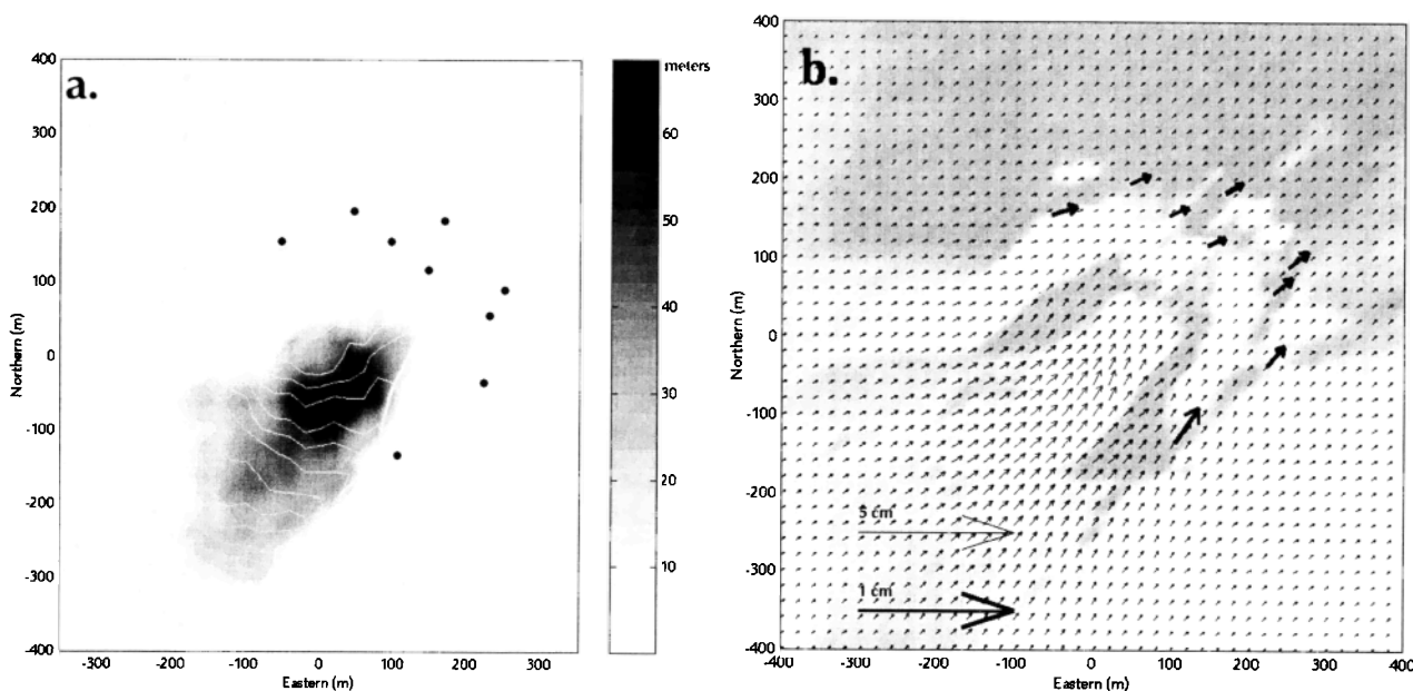
Figure 10. (a) Dome height difference between 1993 and 1994. Black dots are GPS benchmarks. (b) Displacements field due to 1993 to 1994 dome height difference (thin arrows). Heavy arrows represent displacements at GPS benchmarks position (different scale).
