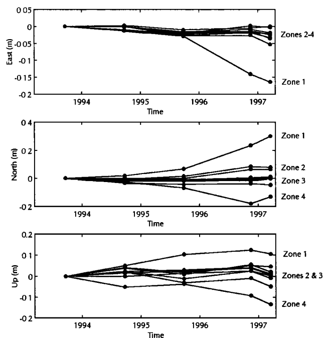
Figure 8. Relative displacements from 1993 to 1997 for each component and corresponding zone number.
