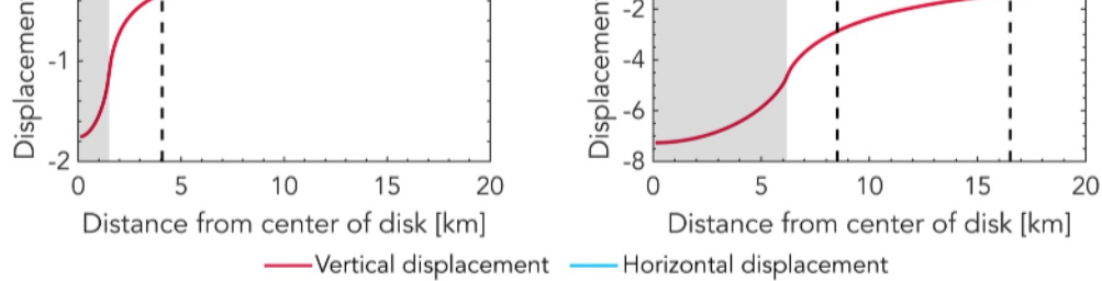
Figure 9. Estimating the elastic loading contribution from a surface water reservoir. (a) Daily and monthly-averaged temporal evolution of water levels at the Harry S. Truman Reservoir. (b) Location of global navigation satellite system (GNSS) stations MOCL and MOWW with respect to the reservoir. (c),(d) Same as Figure 7 and S2 but with projections of the GNSS-Gravity Recovery and Climate Experiment residuals onto reservoir water levels (blue). (e),(f) Displacements associated with the analytical elastic loading model (as in Figure 6a) for the circular regions shown in (b) and a 5m increase in water level.
