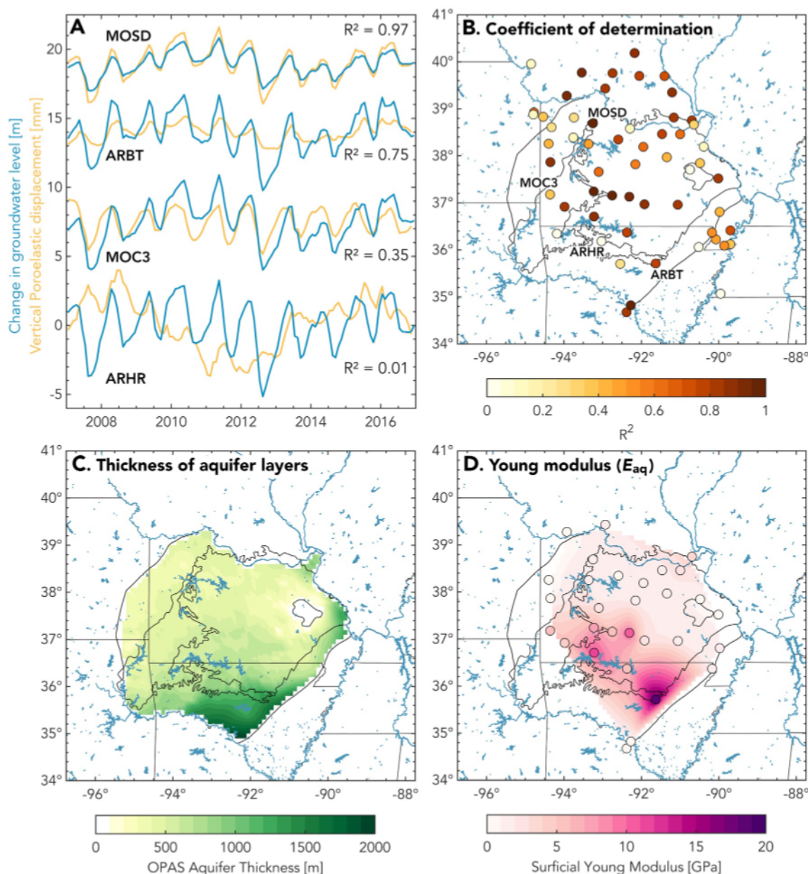
Figure 10. Estimating the aquifer Young modulus from vertical poroelastic displacements and groundwater level variations (a) Examples of vertical poroelastic displacement time series and groundwater level change extracted with independent component analysis and interpolated at the global navigation satellite system stations location. Note that the time series are offsetted for illustration purposes. (b) Coefficient of determination ( R^2 ) of a linear fit through poroelastic displacements versus change in groundwater level. The higher R^2 , the better the E_{aq} estimate. (c) Total thickness of the aquifer layers. (d) Young modulus computed for R^2 > 0.35 and where all three input variables are available.
