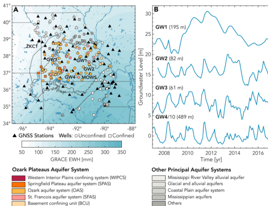
Figure 3. Global navigation satellite system (GNSS), Gravity Recovery and Climate Experiment (GRACE), and groundwater data sets. (a) Annual equivalent water height peak-to-peak amplitudes derived from GRACE and locations of GNSS stations and groundwater monitoring wells used in this study. The color of the well markers indicates the aquifer system at the base of a well and the shape describes the type of aquifer(s)—that is, confined or unconfined—encountered by a well (as classified by the United States Geological Survey [USGS]). (b) Example of groundwater time series at different locations across the Ozark Plateaus Aquifer System. Note that the time series are offset and that GW4 is divided by a factor of 10 for illustration purposes. Well depths are indicated in parenthesis. The featured wells correspond to USGS site numbers 373955091065901 (GW1), 372,853,091,061,801 (GW2), 373,701,093,151,601 (GW3) and 364,324,091,515,001 (GW4).
