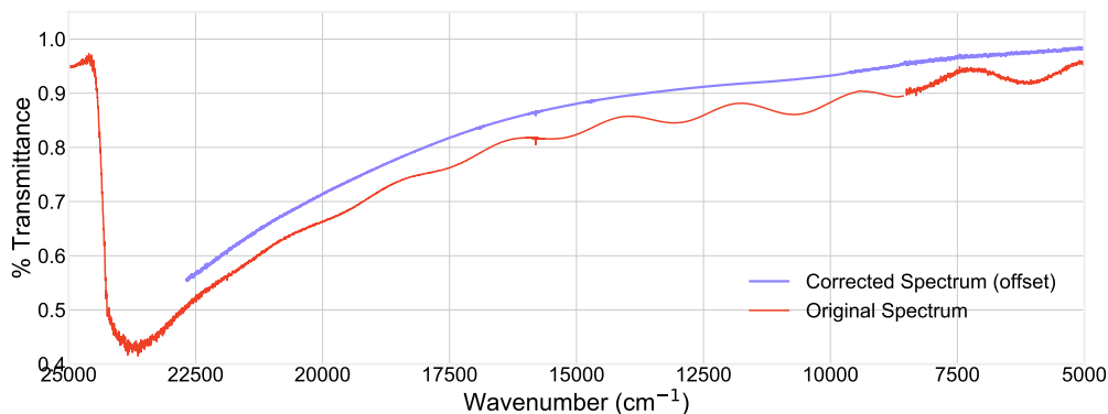
Figure C1. Raw (red) and fringe-corrected transmittance spectrum of the Triton haze analogues.
