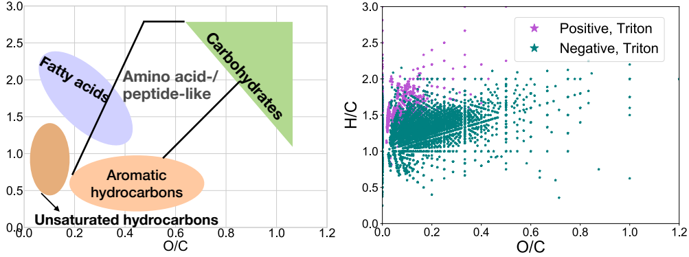
Figure 6. LEFT: An empty van Krevelen diagram showing H/C vs O/C with shaded, labeled regions denoting where particular molecular functional groups tend to cluster, following Ruf et al. (2018). RIGHT: van Krevelen in terms of H/C vs O/C for our Triton sample. The Triton sample clusters strongly in the regions for fatty acids and amino acid-like molecular groups.
