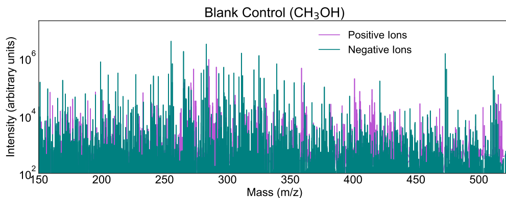
Figure B1. Positive (magenta) and negative (teal) ion mode mass spectra of the blank solution of CH 3 OH from m/z 150 to 525. The blank clearly lacks the structure of the actual sample (see Figure 4). Peaks greater than 2 \times 10^5 present in the blank were removed from the Triton samples before peak assignments were made. These removed peaks constitute less than 0.03% of all peaks.
