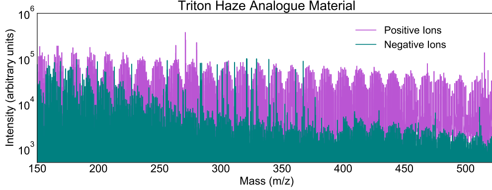
Figure 4. Positive (magenta) and negative (teal) ion mode mass spectra of the Triton haze analogue particles from m/z 150 to 525. Due to differing ionization efficiencies, the negative ion mode intensities are systematically lower. Peak groupings of \sim 13.5 amu repeat across the observed mass range.
