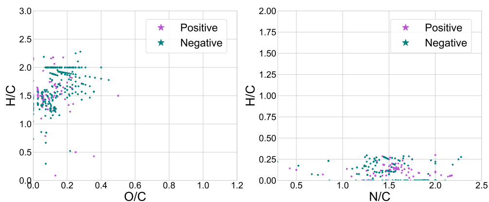
Figure B2. Positive (magenta) and negative (teal) ion mode van Krevelen diagrams of the blank solvent control. Left: H/C vs O/C. Right: H/C vs N/C.
