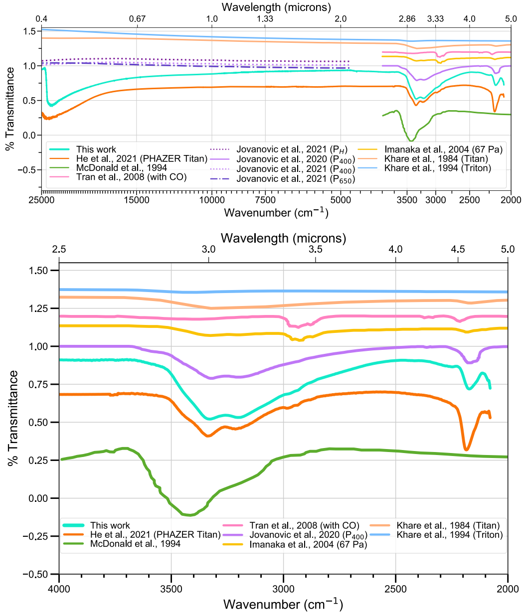
Figure 8. TOP: Transmittance spectra of various tholins produced from \text{N}_2\text{-CH}_4 mixtures. The full details of each experiment can be found in Table 3. Some features are present in all tholin. In the Triton tholin of this work, we attribute some of the broadening and additional absorption between 3500 and 2500 \text{cm}^{-1} to be due uniquely to O-H bonds. These bonds likely result from \text{CO} > \text{CH}_4 in the initial gas mixture. All spectra have been offset vertically for clarity. BOTTOM: As above with emphasis on the 4000 \text{cm}^{-1} to 2000 \text{cm}^{-1} region.
