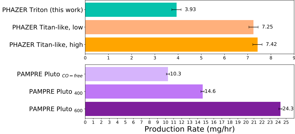
Figure 2. Top: PHAZER production rates (in mg/hr) of the amount of solid produced from the Triton gas mixture ( CO = 0.5\% ; CH_4 = 0.2\% ; top bar in turquoise) compared to our Titan-like tholin ( CH_4 = 5\% ; CO in varying mixing ratios from 0% to 5%; He et al. 2017, middle and lower orange bars). Bottom: PAMPRE production rates from the room temperature Pluto-like tholin ( P_{CO-free} : CO = 0\% , CH_4 = 1\% , top pale purple bar; P_{400} : CO = 500ppm ; CH_4 = 1\% , middle purple bar; and P_{600} : CO = 500ppm , CH_4 = 5\% , lower dark purple bar) of Jovanović et al. (2020). Note that due to differing experimental set-ups, the absolute production rates between the PHAZER and PAMPRE apparatus cannot be directly compared and have different x-axis limits. While CO alters the haze chemistry, higher methane mixing ratios generate larger amounts of haze material in both experimental set-ups.
