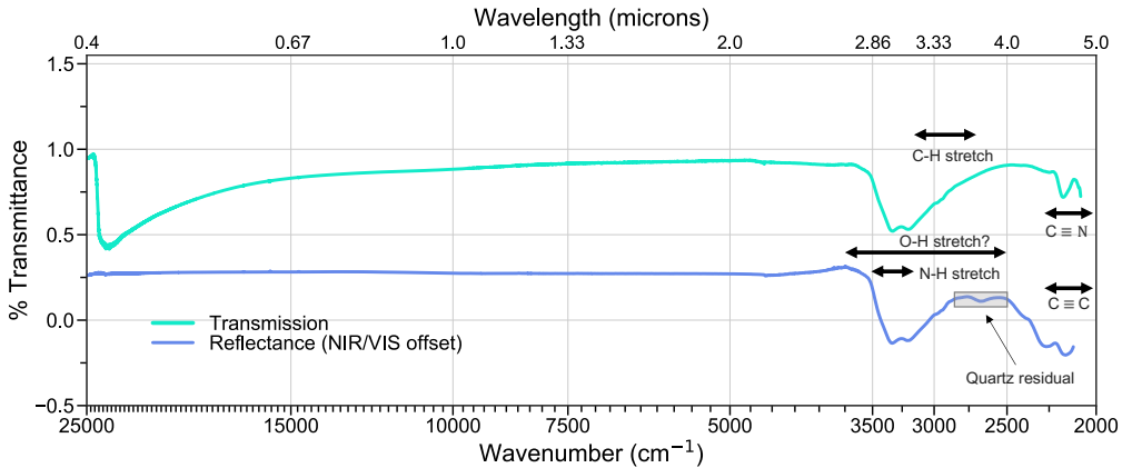
Figure 7. Transmittance (teal) and reflectance (periwinkle) of the Triton tholin. A downward slope is visible from 15000 cm -1 in transmission and features from O-H, N-H, C-H, C=C, and C \equiv N are present from 4000 to 2000 cm -1 in both transmittance and reflectance spectra. The reflectance spectrum has been offset from the transmittance spectrum in the NIR by 0.4 for clarity. Note that the reflectance spectrum contains a residual absorption feature at \sim 2600 cm -1 likely from the quartz substrate.
