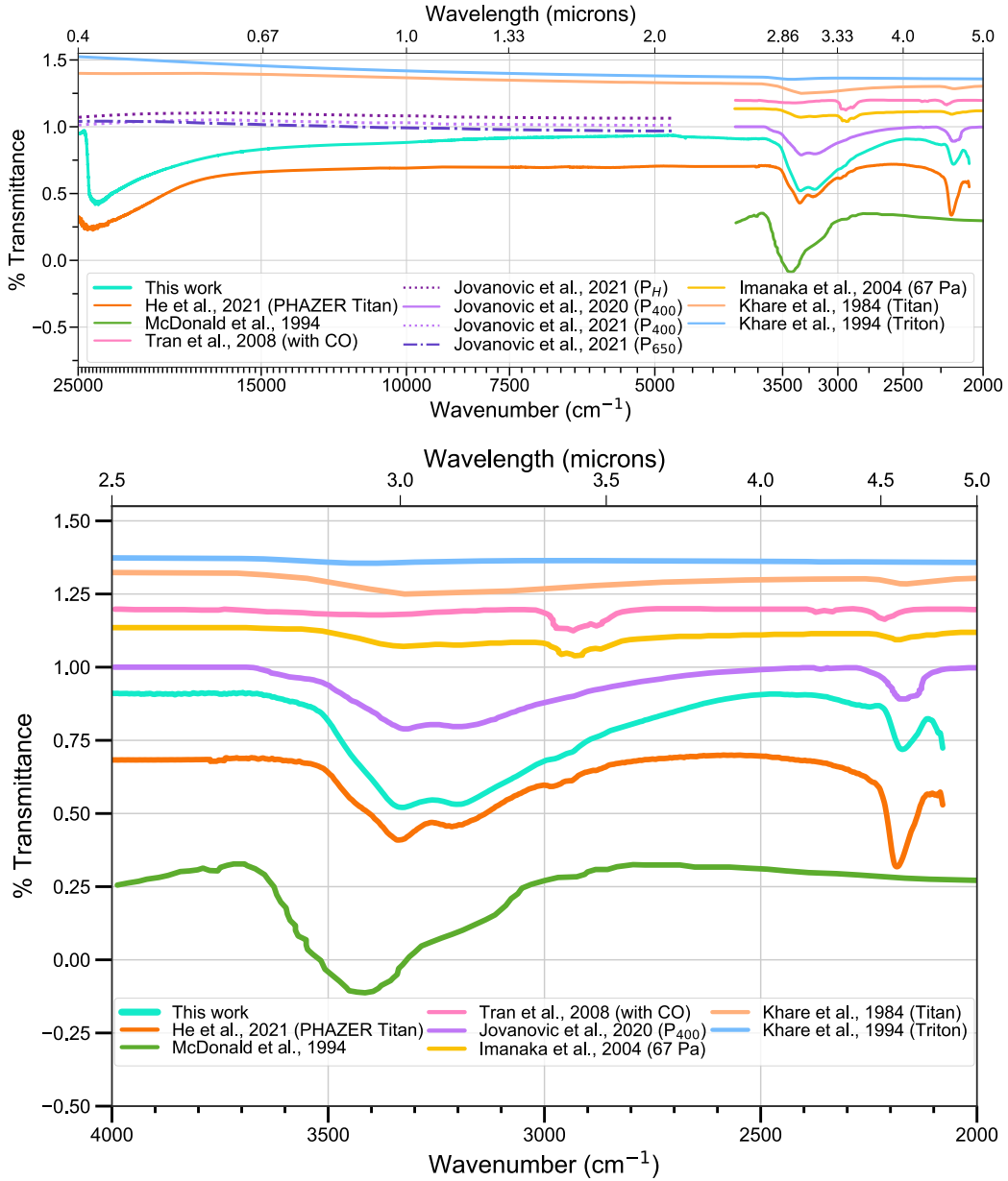
Figure 8. TOP: Transmittance spectra of various tholins produced from N 2 -CH 4 mixtures. The full details of each experiment can be found in Table 3. Some features are present in all tholin. In the Triton tholin of this work, we attribute some of the broadening and additional absorption between 3500 and 2500 cm -1 to be due uniquely to O-H bonds. These bonds likely result from CO > CH 4 in the initial gas mixture. All spectra have been offset vertically for clarity. BOTTOM: As above with emphasis on the 4000 cm -1 to 2000 cm -1 region.
