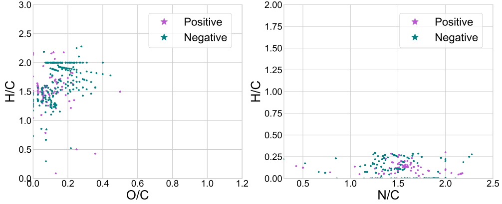
Figure B2. Positive (magenta) and negative (teal) ion mode van Krevelen diagrams of the blank solvent control. Left: \text{H/C} vs \text{O/C} . Right: \text{H/C} vs \text{N/C} .
