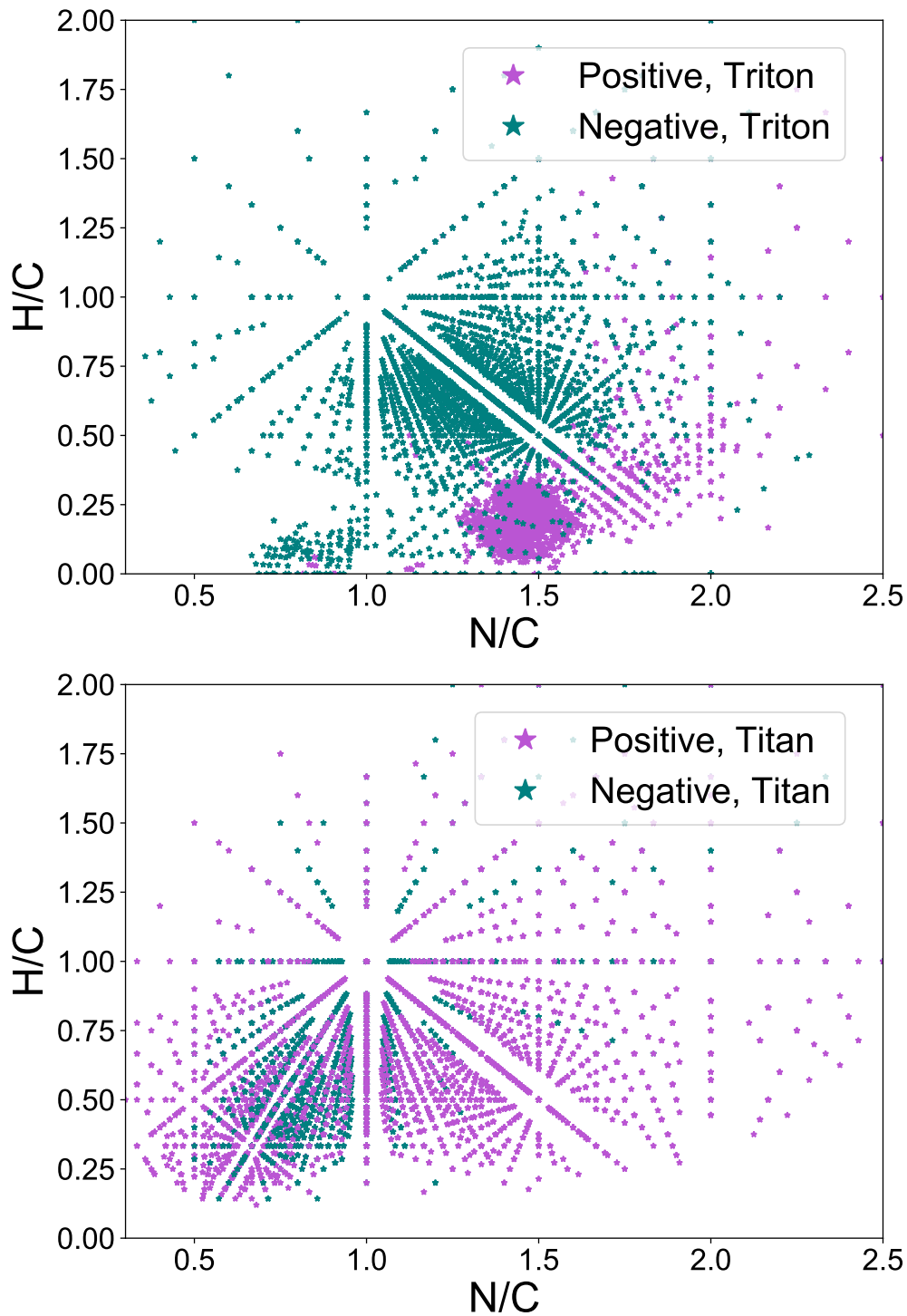
Figure 5. van Krevelen diagrams of the PHAZER Triton haze analogues (top) and PHAZER Titan haze analogues (bottom) in terms of H/C vs N/C, as is common in other tholin studies. The molecular character clearly differs between negative and positive ionizations, underscoring the need for both to understand the sample’s chemistry. The nitrogen incorporation also clearly differs between the Titan sample and the Triton sample produced from a gas mix with CO dominant over CH 4 .
