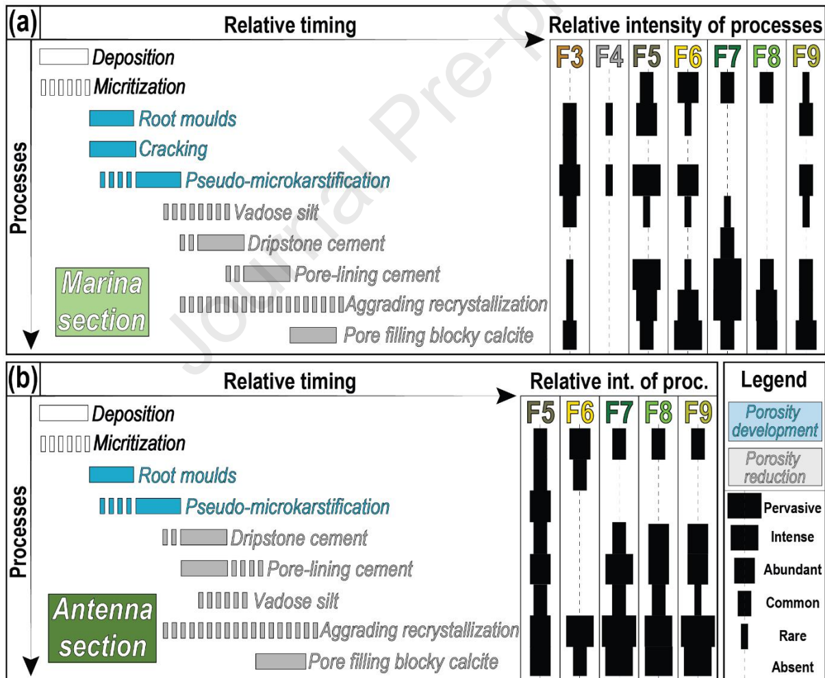
360 Fig. 5. Paragenetic sequences of the studied sections showing the relative intensity of each process sorted per 361 facies: (a) Paragenesis for Marina section; (b) Paragenesis for Antenna Section. The legend explains the color code 362 for porosity development or reduction and the relative intensity scale of the diagenetic processes. 363 364
