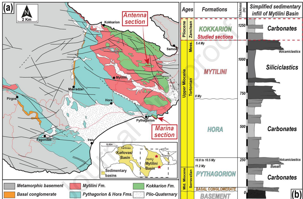
141 Fig. 1. Geological framework: (a) Map of Samos Island (Greece) showing the two sedimentary basins and the two 142 study sites, with a focus on the Mytilini basin; (b) Stratigraphic column of the Mytilini basin (modified after 143 Weidmann et al., 1984; Bailly et al., 2019a). Studied sections are part of the Kokkarion Formation. 144
