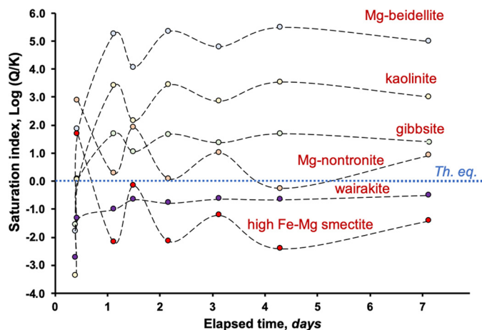
Fig. 9. Temporal evolution of the saturation indices of the reactive fluid during flow-through experiment 3 with respect to selected secondary phases, as calculated with PHREEQC using the Ilnl database. The blue dotted line at SI = 0.0 represents the conditions of thermodynamic equilibrium between the fluid and the solid phases.
