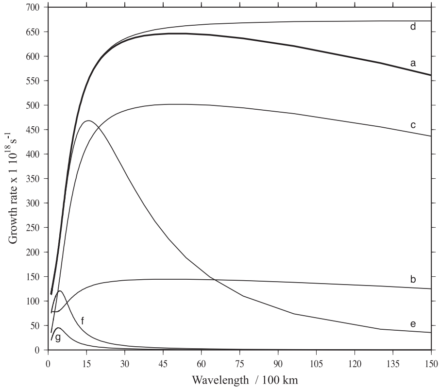
Figure 6. Instability analysis for n = 3 , that is, the lithosphere deforming by plastic creep. (a) reference curve where \eta_1 = 5 \times 10^{22} Pa s, \eta_2 = 10^{18} Pa s, \gamma = 10^{-16} s ^{-1} , \Delta\rho = 1 per cent; (b) idem as (a) but \Delta\rho = 0 per cent; (c) idem as (a) but \gamma = 0 ; (d) idem as (a) but \eta_2 = 10^{16} Pa s; (e) idem as (a) but \eta_2 = 10^{20} Pa s; (f) idem as (a) but \eta_2 = 10^{22} Pa s; (g) idem as (a) but \eta_2 = 5 \times 10^{22} Pa s.
