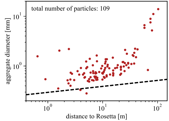
Figure 4. All aggregates with their diameter and distance to the spacecraft. The dashed line is an estimated detection limit derived in Appendix B, smaller particles would be too faint to detect.
