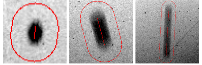
Figure 2. Example of aperture photometry with stadium shape for three different particles. The central lines mark the position of the particle and the beginning of the aperture integration. The stadium shapes mark the mask where we measured the background signal.
