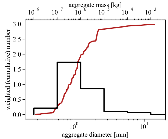
Figure 5. Cumulative (red curve) and histogram (black curve) size distribution of all particles in the analysed sequence.
