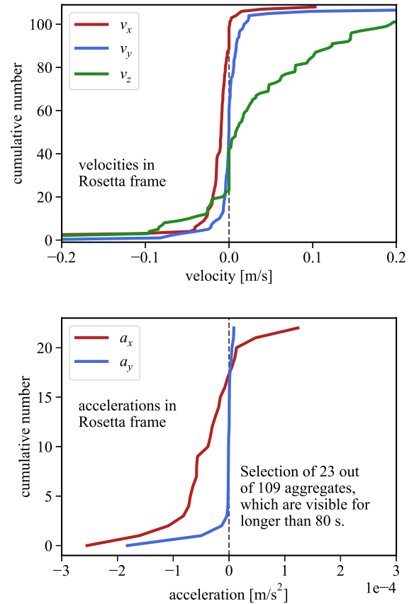
Figure 8. Velocity distribution of all particles (top) and the distribution of accelerations for a subset of particles, which were visible for longer than 80 s (bottom).
