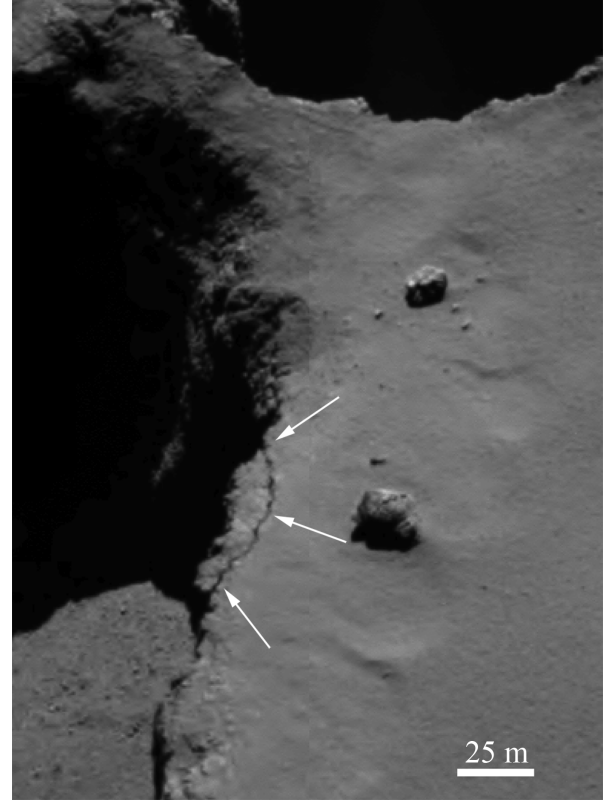
Fig. 11. Fracture of \sim 50 m located at the edge of the Aswan escarpment. The location of this close-up image is indicated in Fig. 7.
