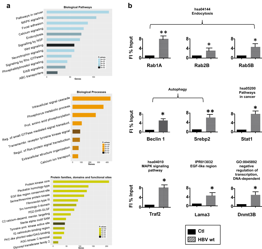
Fig. 1 Functional analysis of protein-coding genes potentially regulated by HBx. a Biological Pathways (KEGG, REACTOME), Biological Processes (GO) and Protein families, domains and important sites (InterPro) over-represented (Benjamini-corrected p -value < 5 \times 10^{-2} ) from the analysis of ~5500 protein-coding genes with HBx-binding sites are shown. In each plot, the categories are in descending order with respect to the associated gene number, with the corresponding color scale of p -values shown on the right. b Validation of HBx occupancy on selected gene promoters in independent ChIP experiments. ChIP results are expressed as Fold Induction (FI) of the % of Input. Histograms show the mean from three independent experiments; bars indicate SD. P -values: * 0.02 \leq P < 0.05 ; ** 0.01 \leq P < 0.02 ; *** 0.005 \leq P < 0.01 . Gene specific promoter primer pairs are detailed in Additional file 1: Table S6
