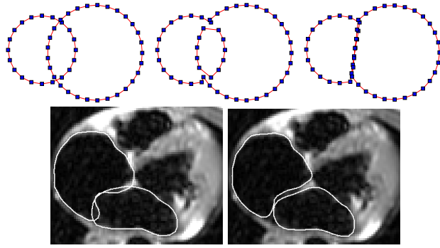
Fig. 5. (from left to right) Two intersecting connected components; after merging the two pairs of intersecting edges; after aligning vertices along the intersecting edges. Example of 2 active contours reconstructing the right and left ventricles in a MR image with a repulsive behavior between each components.
