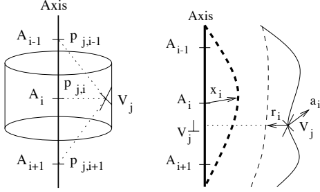
Figure 4. axial forces
