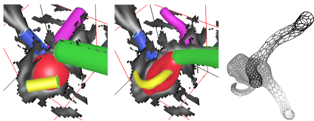
Figure 11. Vessel models
