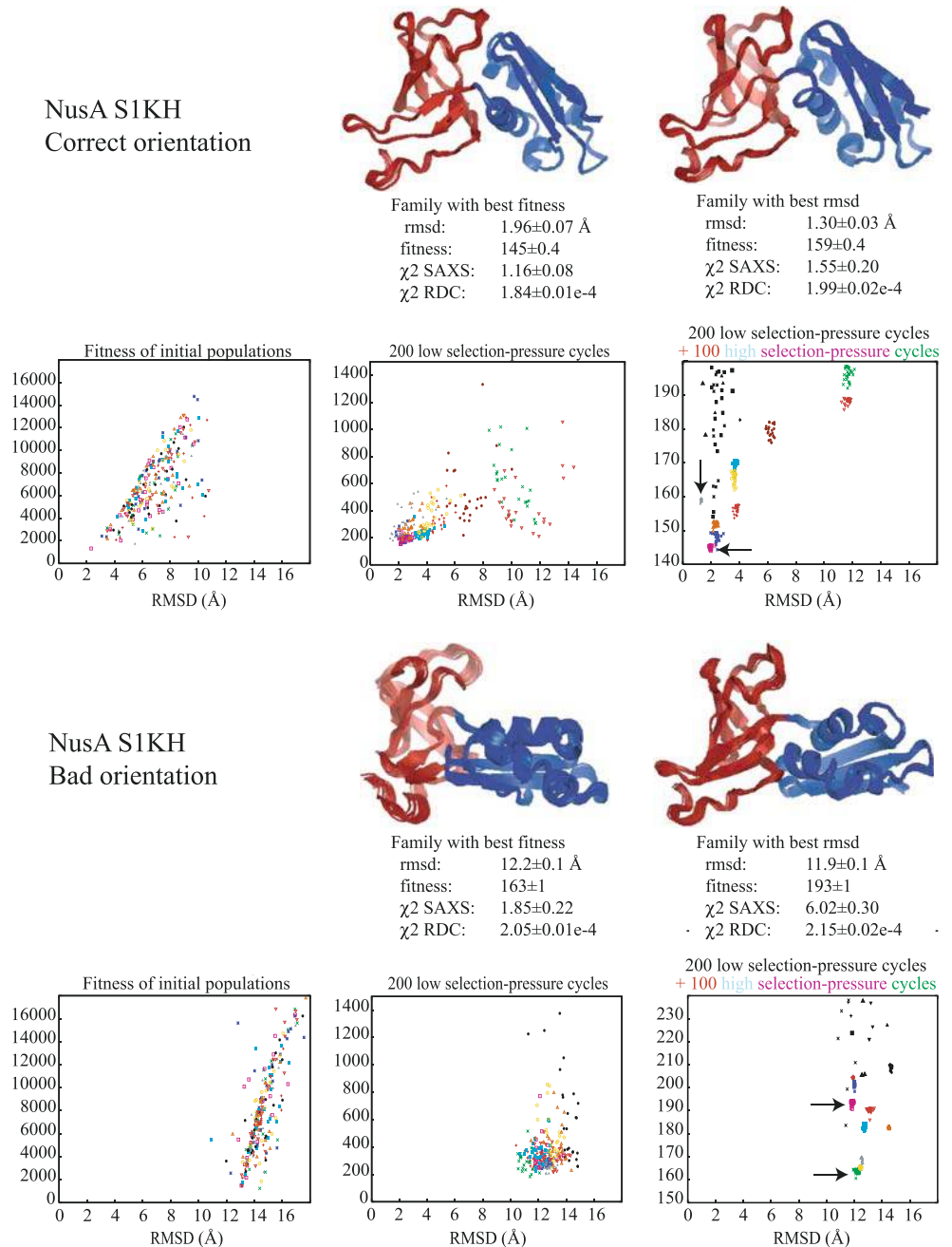
Fig. 4 Results of the genetic algorithm when starting from the crystallographic structures of the domains. The crystallographic structures of the isolated SI and KH domains were used, after randomization of the linker regions, to form the initial populations as described in the text. Upper part the two domains are oriented like in the target structure. Lower part the KH domain is orientated with a 180° rotation around the y-axis. For each orientation, we displayed the families with the best fitness and with the best rmsd. We plotted the fitness versus the rmsd to the target in the initial population ( left plot ), at the end of the 200 first generations ( middle plot/color symbols ; right plot/black symbols ) and after 100 supplementary generations with high selection-pressure ( right plot/color symbols ). The displayed families are indicated by arrows
