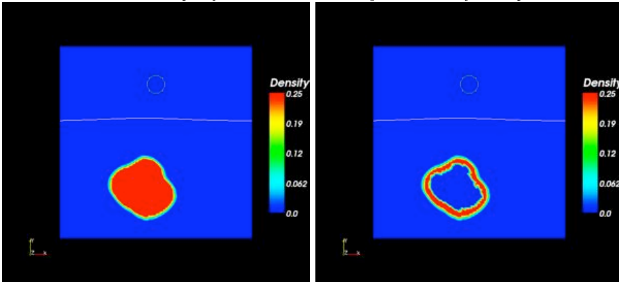
FIG. 4.3. Total and proliferative tumoral density at the end of the experiment.
