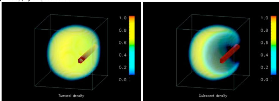
FIG. 4.6. Total and quiescent density of the tumoral cells at the end of the experiment. The oxygen supply is plotted in red.
