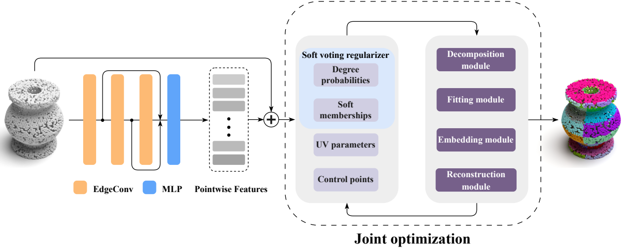
Figure 1: Overview of the proposed pipeline. The network takes a point cloud as input. It outputs pointwise features followed by four modules to predict Bézier geometry and topology: (1) The decomposition module decomposes point clouds into multiple patches. (2) The fitting module regresses uv parameters for each point and control points for each Bézier patch. (3) The embedding module clusters pointwise features assigned to the same patch. (4) The reconstruction module re-evaluates the input point clouds from the above predictions.
