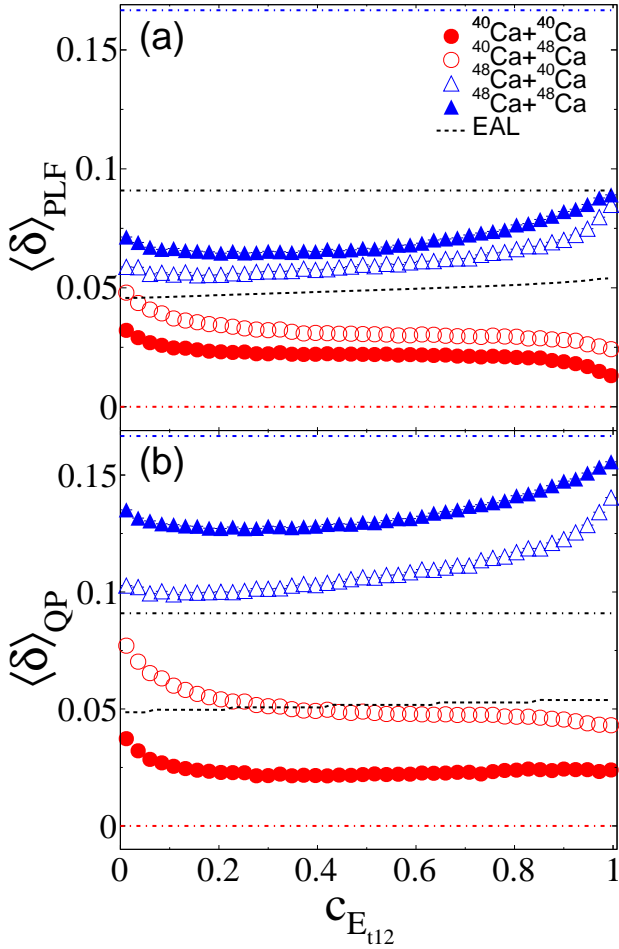
Figure 3: (Color online) Distribution of the average asymmetry \delta as a function of the experimental centrality c_{E_{t12}} for (a) the PLF and (b) the reconstructed QP for the four systems under study. Statistical error bars are smaller than the symbols. The initial asymmetries of the colliding systems and the EAL extracted from [30] (using the average charge of the symmetric systems for each bin of c_{E_{t12}} ) are represented by dotted-dashed and dashed lines, respectively.
