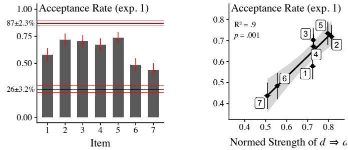
Figure 3: Left: Acceptance rate per item and standard error. The top (respectively bottom) horizontal lines indicate the levels of valid (respectively invalid) controls and the standard errors. Right: Correlation between the average reported strength of the crucial dependence d to a from the norming study ( x -axis) and the acceptance rate of target fallacies in the inference-making task ( y -axis). We plot each individual item. Horizontal and vertical bars indicate the standard error.
