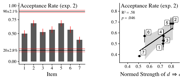
Figure 4: Left: Acceptance rate per item and standard error. The top (respectively bottom) horizontal lines indicate the levels of valid and (respectively invalid) controls and the standard errors. Right: Correlation between the average reported strength of the crucial dependence d to a from the norming study ( x axis) and the acceptance rate of target fallacies in the inference-making task ( y axis; exp. 2). We plot each individual item. Horizontal and vertical bars indicate the standard error.
