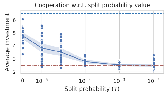
Figure 5: Evolution of cooperation with partner choice for a population size of 1000 robots and a mutation strength for the investment gene \sigma_x = 0.1 . For each setup, 24 independent runs are performed. Results are compiled from 144 runs obtained from 6 different experimental setups. For each setup, learning is performed for 200 generations with a given split probability \tau (x-axis). The values for \tau are: 0, 10^{-5} , 5 \times 10^{-5} , 10^{-4} , 10^{-3} , 10^{-2} . In addition, the blue line shows the average values for each setup with its 95% confidence interval.
