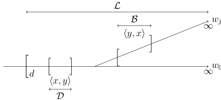
Figure 14: Non-decidedness
