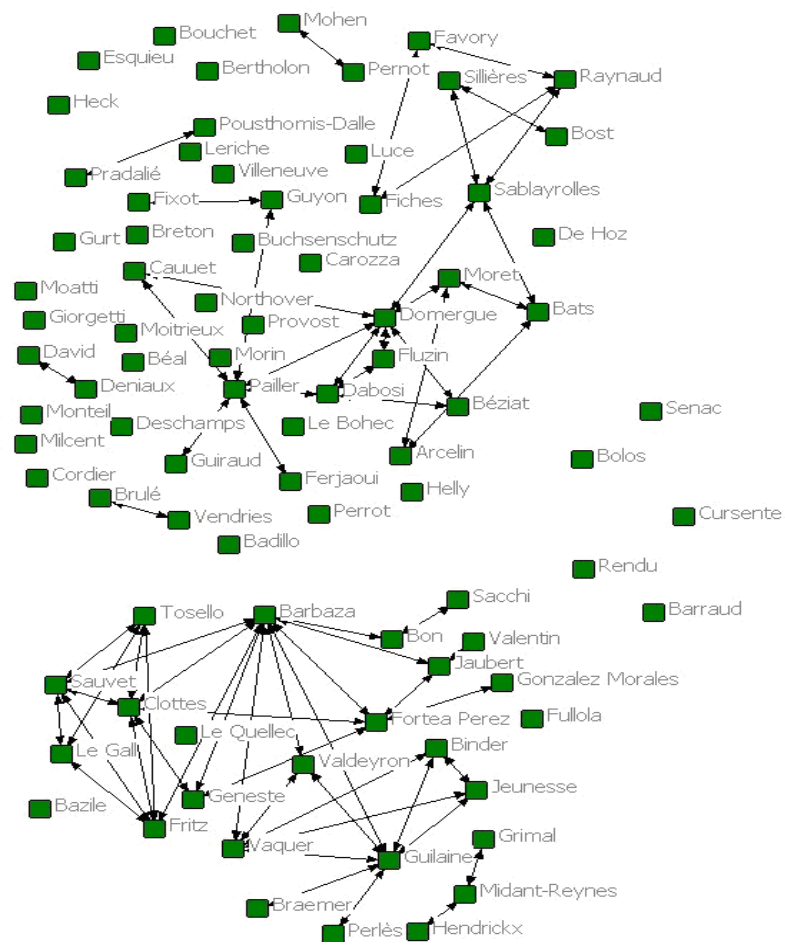
Figure 7. Committee co-membership and co-publication network in archaeology.
