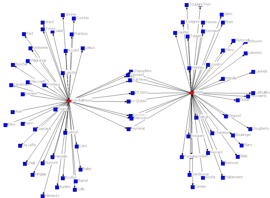
Figure 4. Graph of the co-membership ties of the two most central committee members
