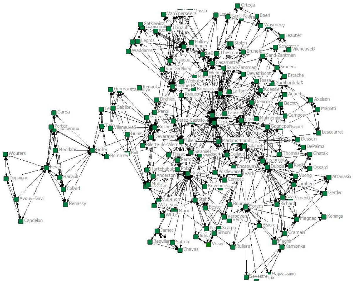
Figure 8. Committee co-membership network in economics
