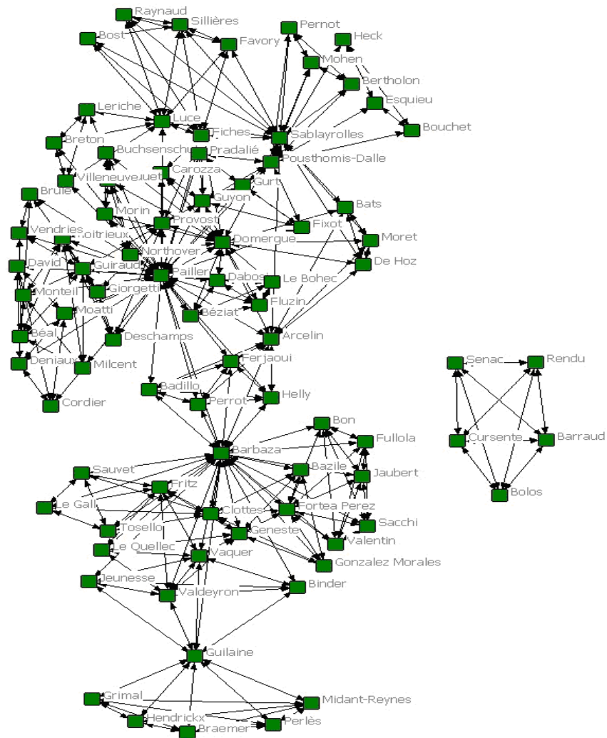
Figure 5: Committee co-membership network in archaeology
