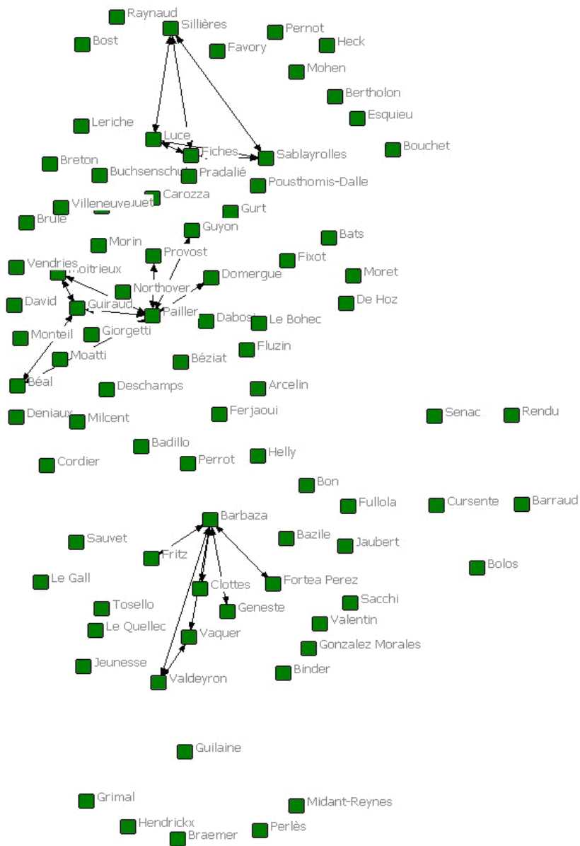
Figure 6: Network of co-membership on, at least, two thesis committees in archaeology:
