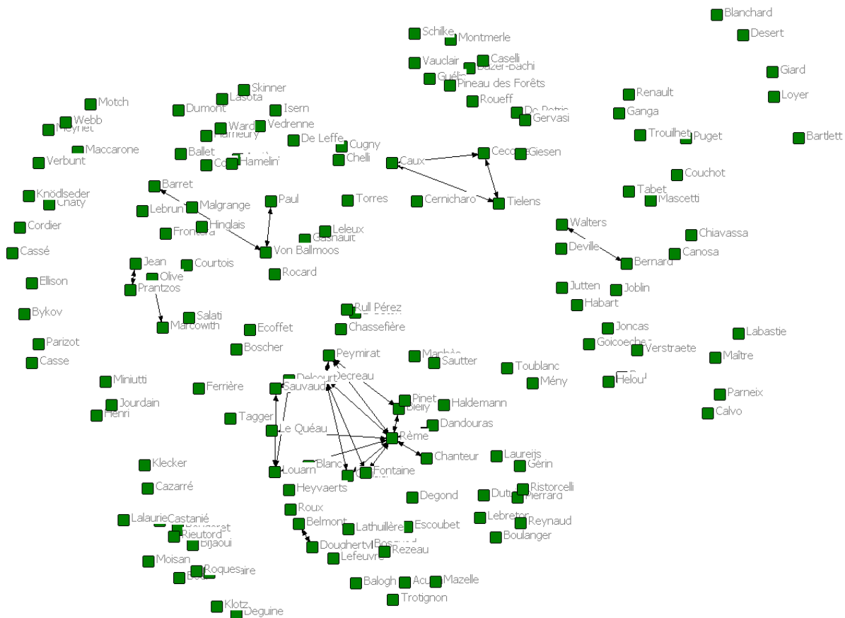
Figure 3. Network of committee co-membership on a minimum of two thesis committees in astrophysics
