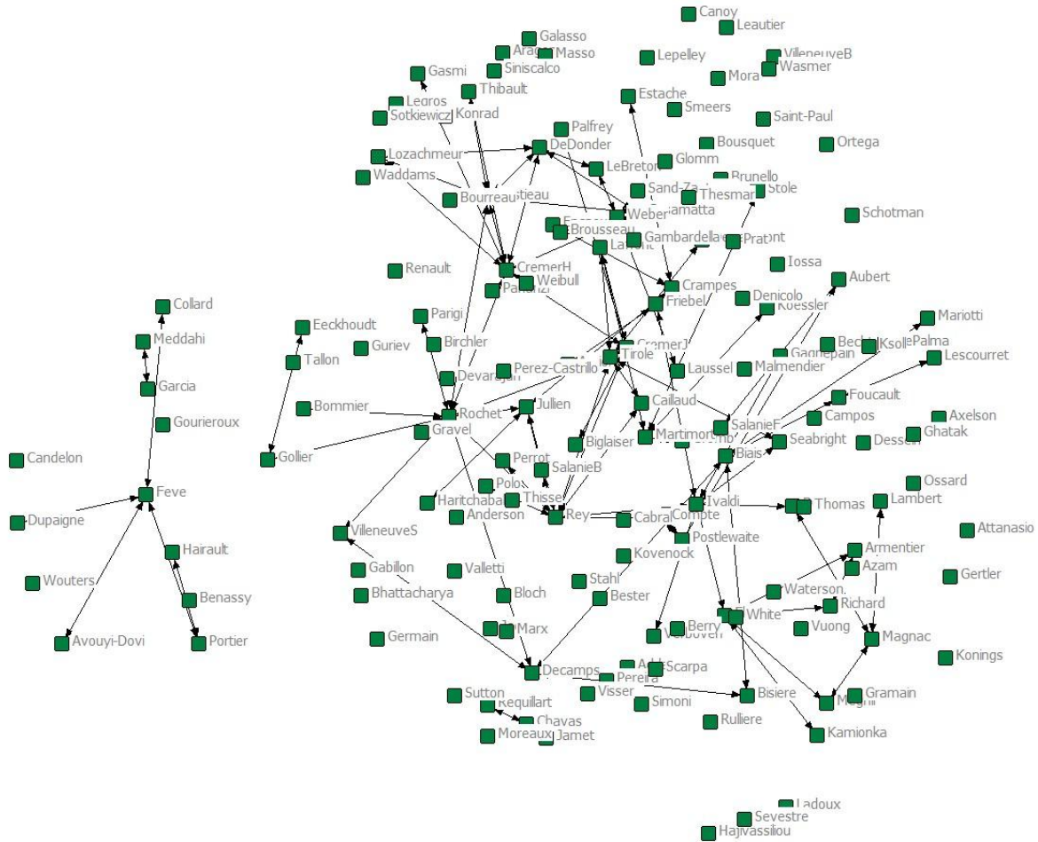
Figure 10. Co-publication and committee co-membership network in economics
