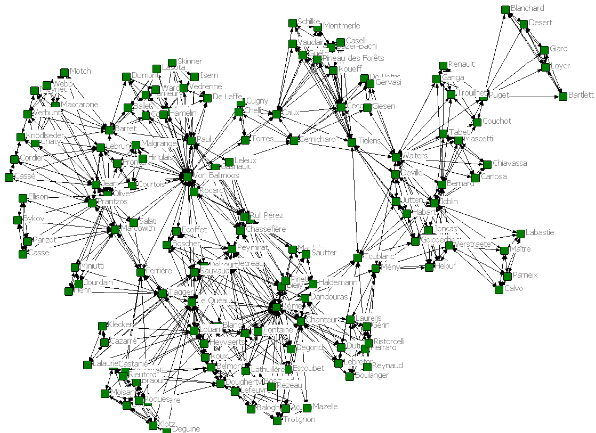
Figure 1. Co-membership in astrophysics
