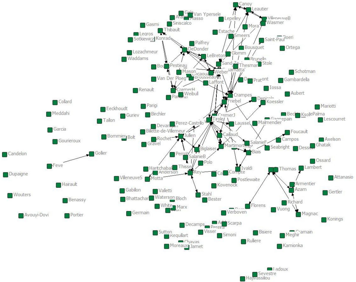
Figure 9. Network of co-membership on, at least, two thesis committees in economics:
