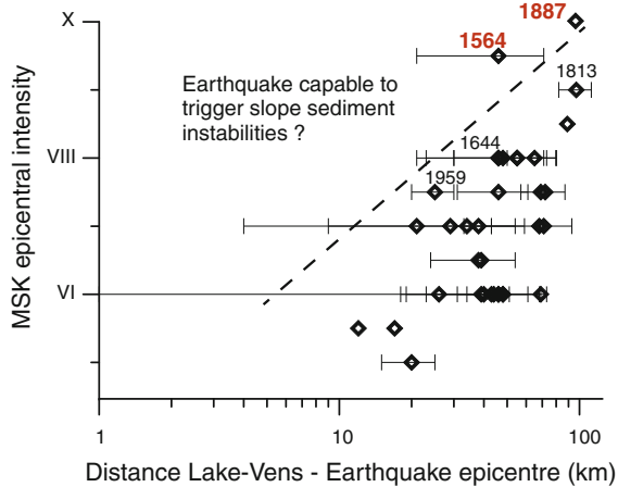
Fig. 8 Intensity versus distance diagram (MSK intensity > V and distance < 110 km) for historic earthquakes near Lake Vens. The dashed line represents the possible seismic sensitivity of Lake Vens. Dates of historic earthquakes that are probably associated with the two most recent H layers are marked in red
